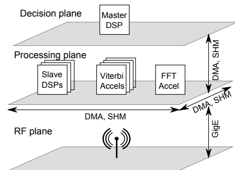
Figure 3: OpenRadio basestation internals with different kinds of compute cores and an RF frontend.
