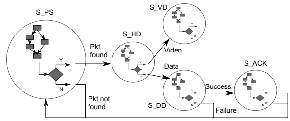
Figure 2: A state machine with states for packet search (S_PS), header decode (S_HD), video decode (S_VD), data decode (S_DD) and sending an acknowledgement (S_ACK).
