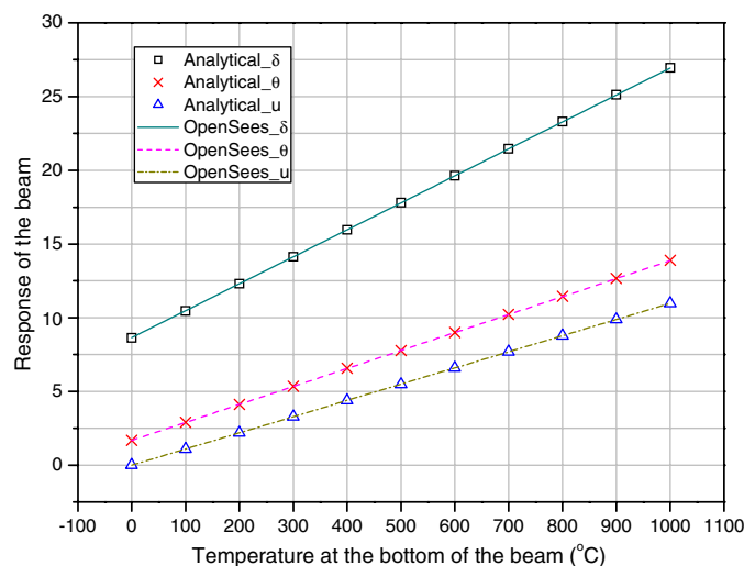
Fig. 13. Responses of the beam from OpenSees compared with analytical solutions ( \delta , u :mm; \theta : 10^{-3} rad)
