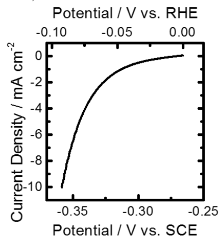
Figure 1. Cathodic polarization behavior of a CoP film in 0.500 M H 2 SO 4 (aq).
