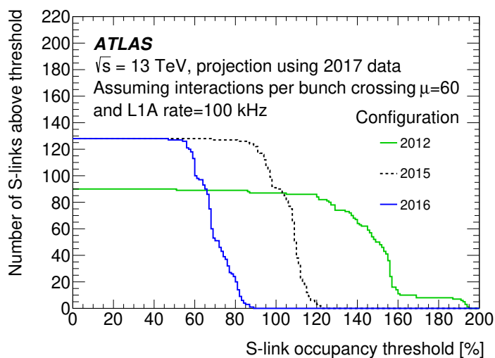
Figure 6: Number of S-links operating above the bandwidth occupancy threshold specified on the x -axis. During operation, once the S-link occupancy exceeds 90% of its bandwidth, the corresponding ROD starts to fall into the busy state, so that it becomes impossible to transfer data correctly. The bandwidth occupancy of each configuration in 2012 (green line, right), 2015 (dashed black, middle) and 2016 (blue, left) is simulated using the extreme condition of a level-1 trigger rate of 100 kHz with \mu = 60 . The line labelled 2012 shows the 90-ROD system used in Run 1, where many S-links were not able to handle the high data rate. Several S-links for endcap modules showed significantly higher occupancy than the other S-links, due to an imbalanced distribution of data rate per ROD. These features were significantly improved in the 2015 configuration with 128 RODs. In 2016 the supercondensed mode was introduced and the FE-link remapping was performed, in order to distribute the S-link occupancy more uniformly.
