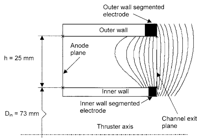
FIG. 1. Schematic of the thruster channel of a 2 kW segmented Hall thruster with superimposed magnetic field lines. The magnetic field distribution was simulated for the experimental conditions. A 4-mm-long inner and 6-mm-long outer segmented electrodes are made of carbon velvet material.
