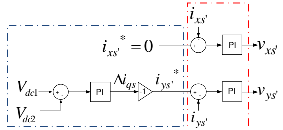
Fig. 4. Structure of the x'-y' current controllers (dotted box on the right) and dc-link voltage balancing controller (dotted box on the left).
