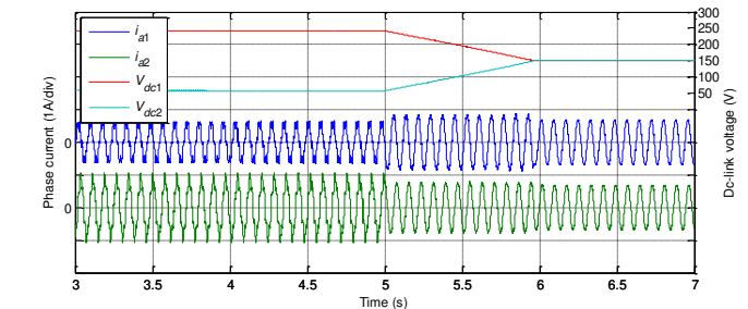
Fig. 17. Simulation results for no-load operation at 250 rpm, showing the activation of dc-link voltage balancing controller at t = 5.0 s.
