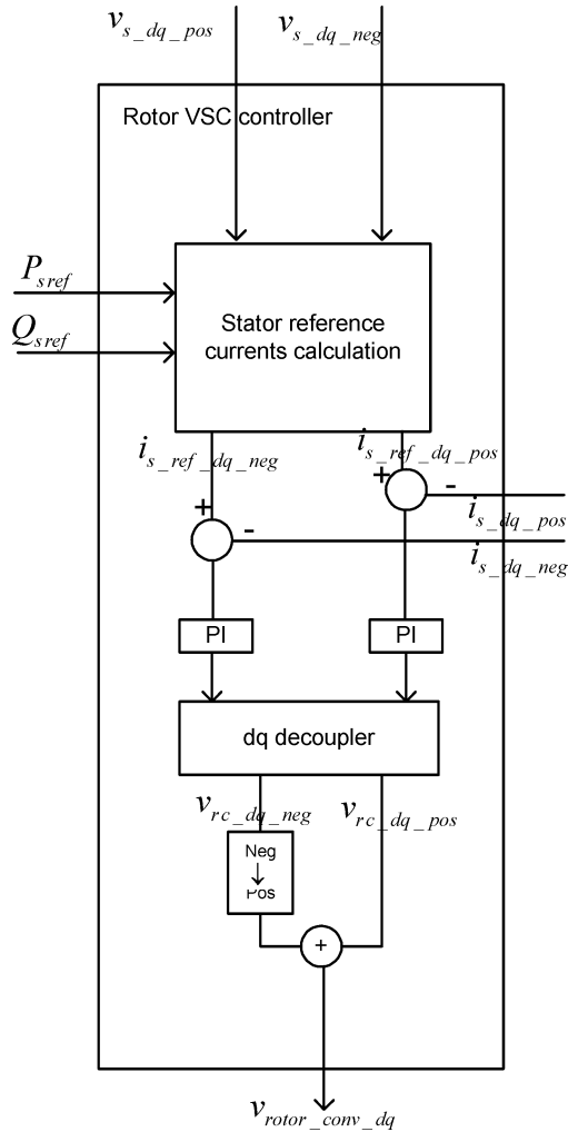
Fig. 9. Dual sequence current controller of rotor VSC.
