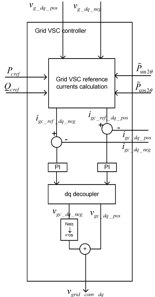
Fig. 10. Dual sequence current controller of grid VSC.
