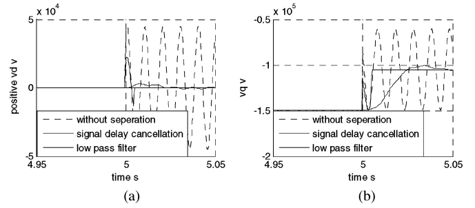
Fig. 8. Unbalanced voltages in positive dq reference frame with and without using the two separation methods (a) v_d and (b) v_q .
