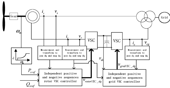
Fig. 1. Simplified diagram of DFIG system with proposed controllers.
