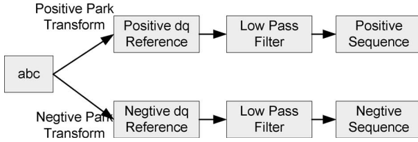
Fig. 6. Separate positive and negative sequences by low-pass filters.
