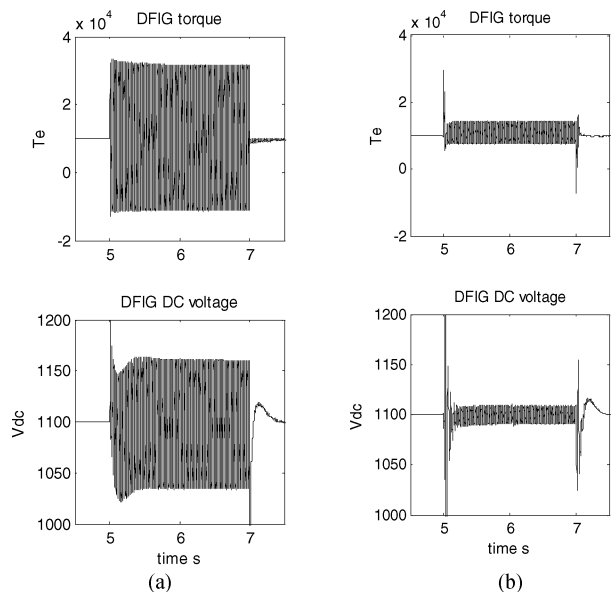
Fig. 11. Compare the responses of DFIG under unsymmetrical voltage dip from different controllers. (a) Single sequence FOC controller. (b) Dual sequence FOC controller. Graphs from top to bottom are electric torque T_e and dc voltage V_{dc} , respectively.
