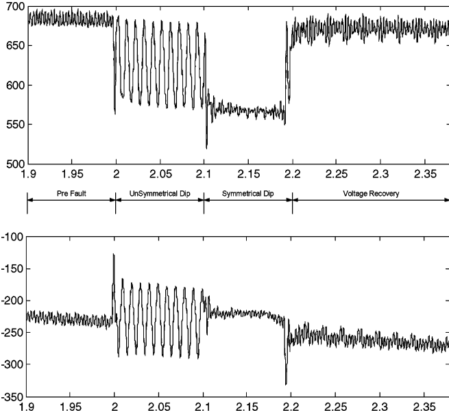
Fig. 4. Stator voltage dips of DFIG.
