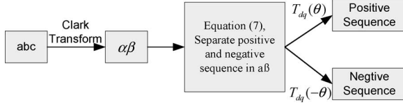
Fig. 7. Separate positive and negative sequences by “signal delay cancellation” method.
