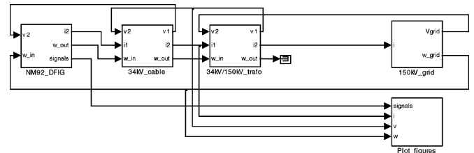
Fig. 3. Simulink model of DFIG system.
