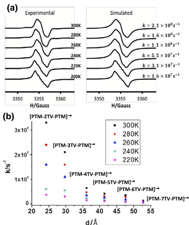
Figure 1: a) Temperature-dependent changes in the EPR spectrum of [PTM-3TV-PTM] •- NBu 4 + solution in CH 2 Cl 2 (left), obtained by chemical reduction with NBu 4 + OH - , and simulated spectra (right) with different spin/charge exchange rates. b) Distance dependences of spin/charge exchange rates, k , of radical-anions [PTM- n TV-PTM] •- in the temperature range 220-300 K.
