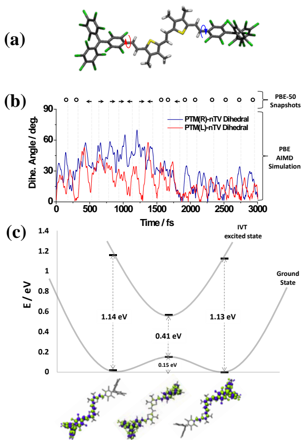
Figure 3: a) Optimized structure of [\text{PTM-2TV-PTM}]^{\bullet-} . The helical arrows indicate the dihedral angles ( \varphi ) between each PTM unit and the 2TV wire. b) Variation of the indicated dihedral angles in a) during 3 ps of an AIMD simulation of [\text{PTM-2TV-PTM}]^{\bullet-} at 300K using the PBE functional. The left/right arrows and circles indicate left/right localization or delocalization of spin density respectively for particular tested snapshots with the PBE-50 functional, c) Relative energies for each studied electronic configuration (left-localized, delocalized and right-localized) in the corresponding relaxed conformations as obtained by PBE-50 optimizations. The calculated energies of the optical IVT (represented by the \beta -HOMO/ \beta -SUMO gap) for each case are also provided. The structures of each configuration with the corresponding highlighted spin densities are provided below the x axis of Figure 3c.
