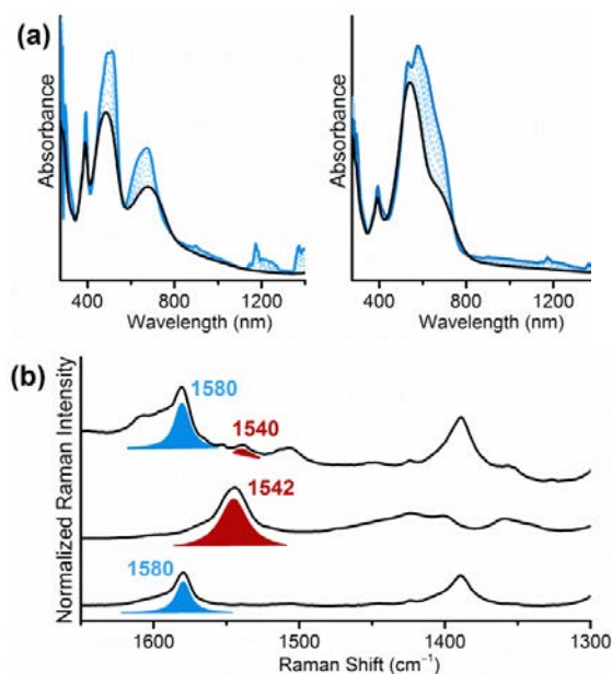
Figure 2: a) Evolution of UV-Vis-NIR spectra of the [PTM-2TV-PTM] •- NBu 4 + (left) and [PTM-5TV-PTM] •- NBu 4 + (right) as a function of the temperature, obtained by chemical reduction with NBu 4 + OH - . Solid black line corresponds to UV-Vis-NIR at room temperature and solid blue line at 77K. b) Comparison of 633nm Raman spectra in DCM of [PTM-4TV-PTM] •- NBu 4 + (top), [PTM-4TV-PTM] •+ Cl - (medium) and [PTM-4TV-PTM] • (bottom).
