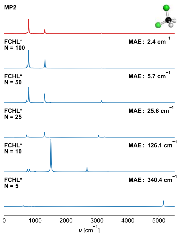
FIG. 9. The unscaled infrared spectrum of dichloromethane calculated via vibrational analysis. (Top/red) Calculated at the MP2/def2-TZVP level of theory; (bottom/blue) using QML to calculate the necessary derivatives of the energy with respect to the nuclear coordinate and the dipole moment. The spectra are convoluted using Lorentzian distributions 69 with a width of \gamma = 8 \text{ cm}^{-1} .
