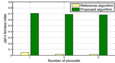
Fig. 4. Jain's fairness index of SSUE versus number of picocells.
