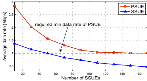
Fig. 2. Average data rate versus number of SSUEs.
