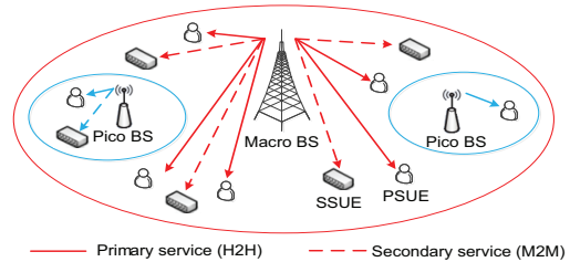
Fig. 1. Opportunistic user association in multi-service HetNets.
