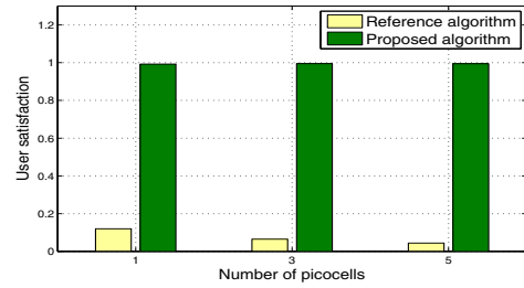
Fig. 3. Average satisfaction of PSUE versus number of picocells.
