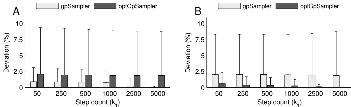
Figure 6. xy -deviation for E. coli iAF1260 xy -deviation from samples obtained with sampler x at step count k_1 to sampler y using k_2=5000 . (a) Deviation to samples obtained by y=gpSampler . (b) Deviation from samples obtained by y=optGpSampler . Self-deviation ( x = y ) is small for both samplers, but there is a large cross-deviation ( x \neq y ). For this large network, we do not observe convergence of gpSampler to the samples obtained by optGpSampler or vice versa as in Fig. 4.
