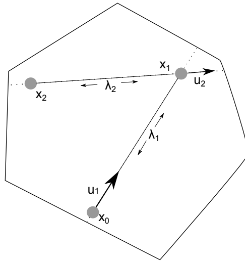
Figure 1. Illustration of hit-and-run
