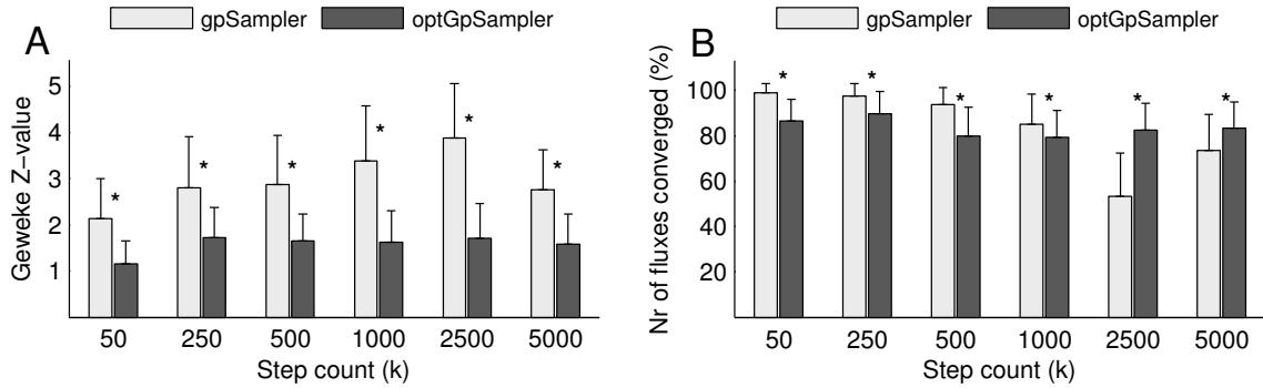
Figure 5. Empirical convergence for E. coli iAF1260. (a) Convergence according to the Geweke diagnostic. (b) Convergence according to the Heidelberger-Welch diagnostic. For both convergence tests, gpSampler 's performance deteriorates when the step count is increased up to k=2500 . Especially the good scores at low values of k seem unrealistic and could indicate convergence towards a non-uniform distribution. Results for optGpSampler seem more stable and more reliable.
