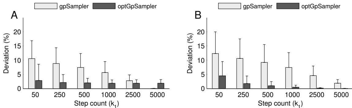
Figure 4. xy -deviation for C. thermocellum iSR432. xy -deviation from samples obtained with sampler x at step count k_1 to sampler y using k_2=5000 . (a) Deviation to samples obtained by y=gpSampler . (b) Deviation from samples obtained by y=optGpSampler . In both cases optGpSampler converges much faster to sampler y .
