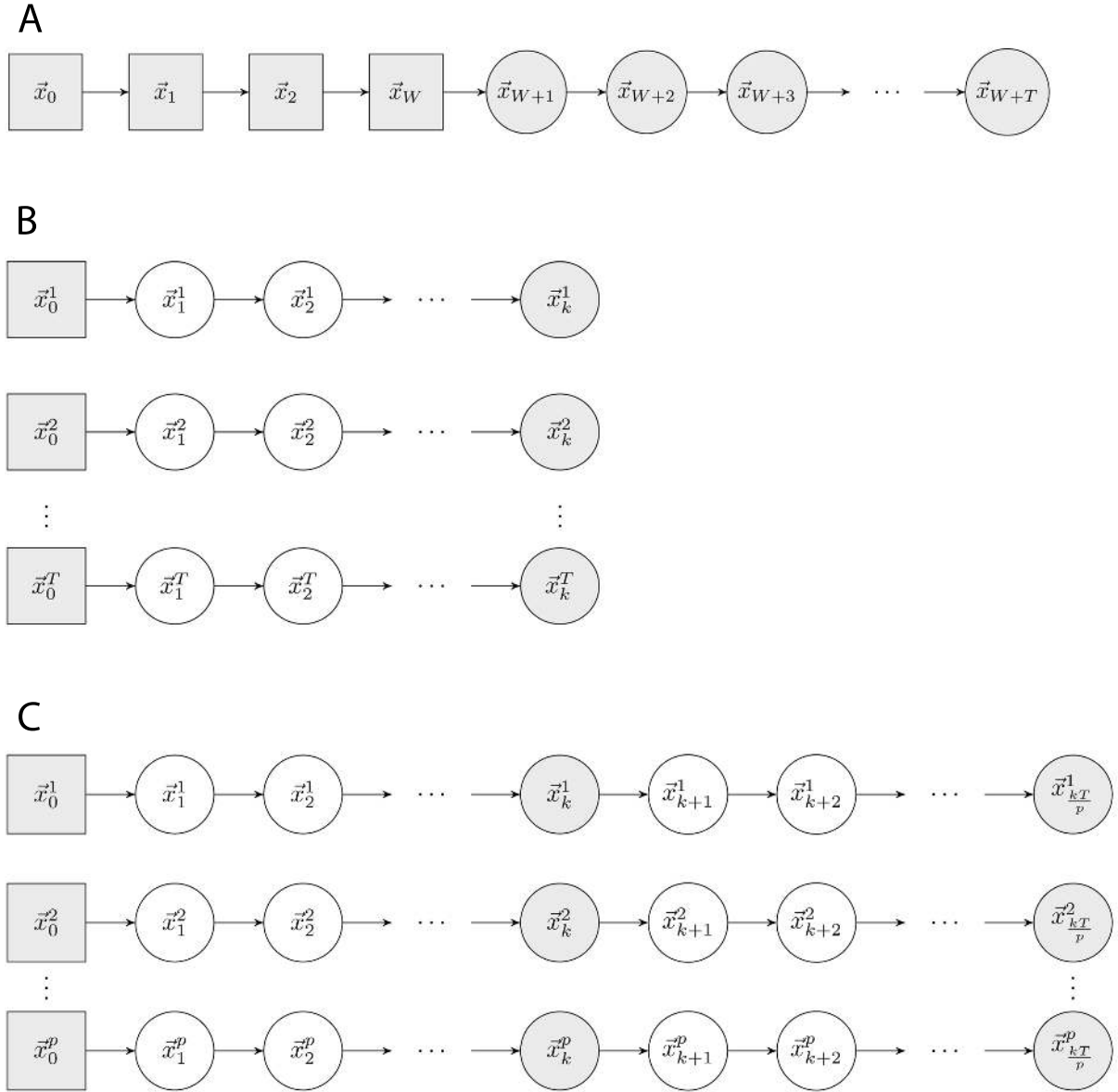
Figure 2. Conceptual difference between the samplers
