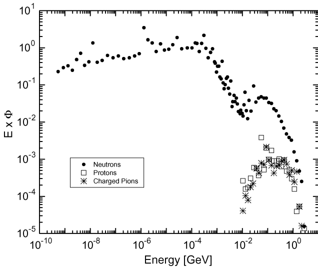
Fig. 2. Lethargy plot of the energy spectrum in the high energy radiation test facility at CERN. Normalization is to 100 keV neutrons.
