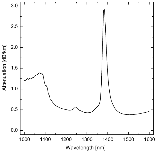
Fig. 4. Attenuation spectrum of the un-irradiated F-doped SM core fiber ⑦.
