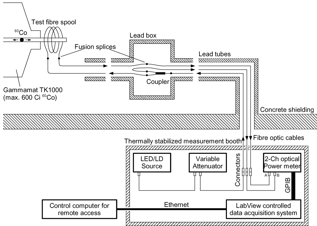
Fig. 1. Experimental setup at the ^{60}\text{Co} irradiation facility at Fraunhofer INT to measure RIA in various fiber samples on-line.
