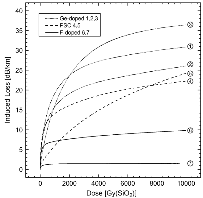
Fig. 5. RIA in the initial sample screening test ( 60 Co source).
