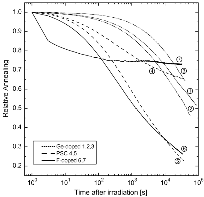
Fig. 6. Annealing (normalized to total induced loss) of the RIA after gamma ray irradiation.
