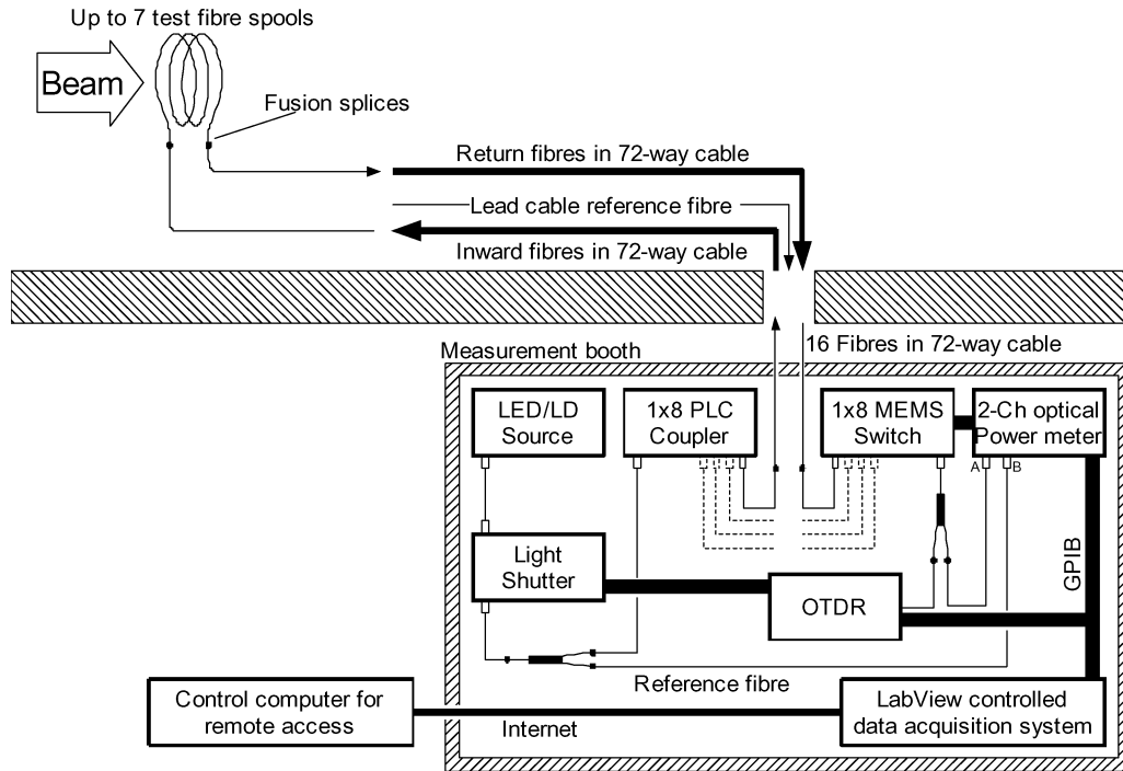
Fig. 3. Experimental setup to measure RIA in various fiber samples on-line (high energy radiation field of the Super proton Synchrotron at CERN).
