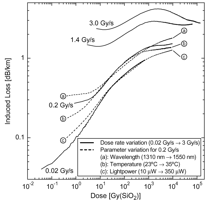
Fig. 8. Dependence of the RIA on irradiation conditions (F-doped fiber ⑦).
