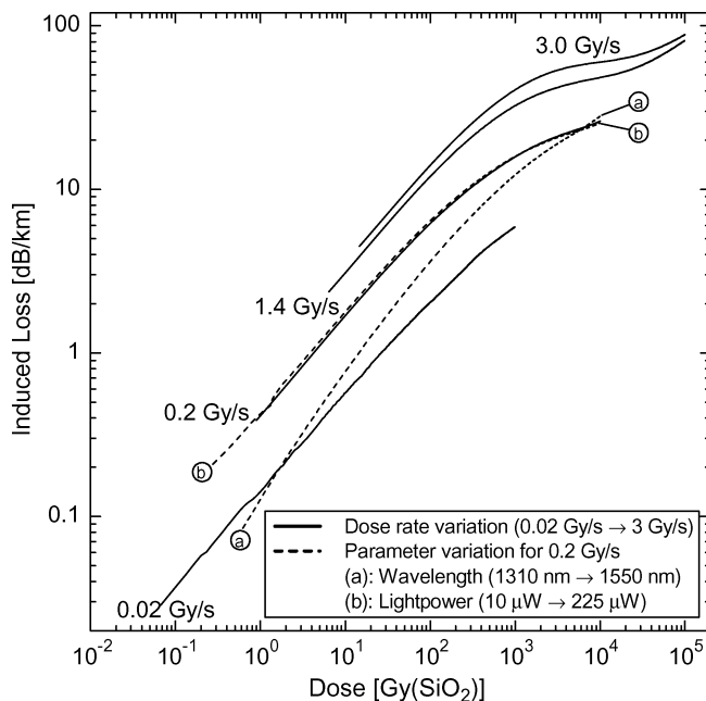
Fig. 7. Dependence of the RIA on irradiation conditions (Ge-doped fiber ②).
