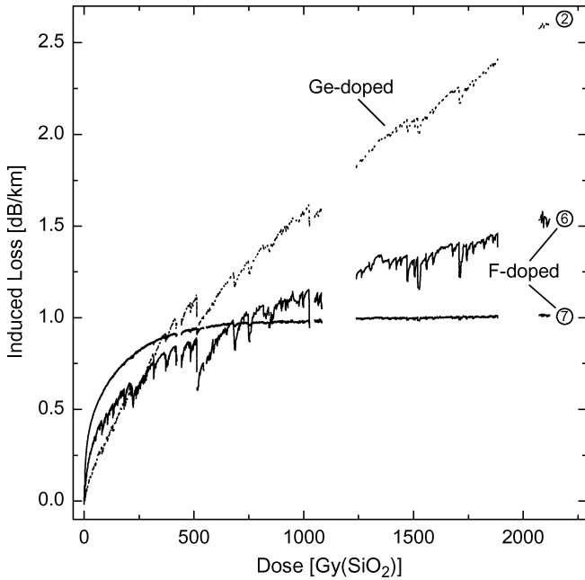
Fig. 9. RIA of the fiber samples in a high energy physics radiation field.
