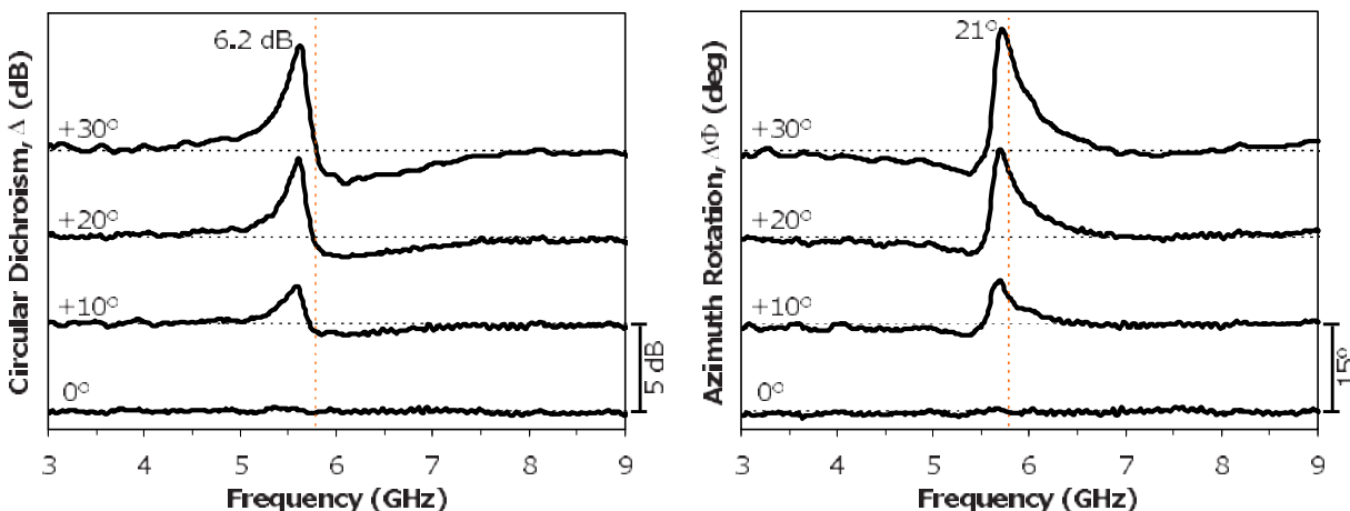
FIG. 3. (Color online) Circular dichroism and birefringence in the non-chiral planar metamaterial structure measured for tilt angles from \alpha = 0^\circ to +30^\circ in steps of 10^\circ . Tilt angles of opposite sign result in reversed signs of circular dichroism and azimuth rotation. The frequency at which pure optical activity on a background of vanishing anisotropy can be seen is marked by a vertical dashed line.
