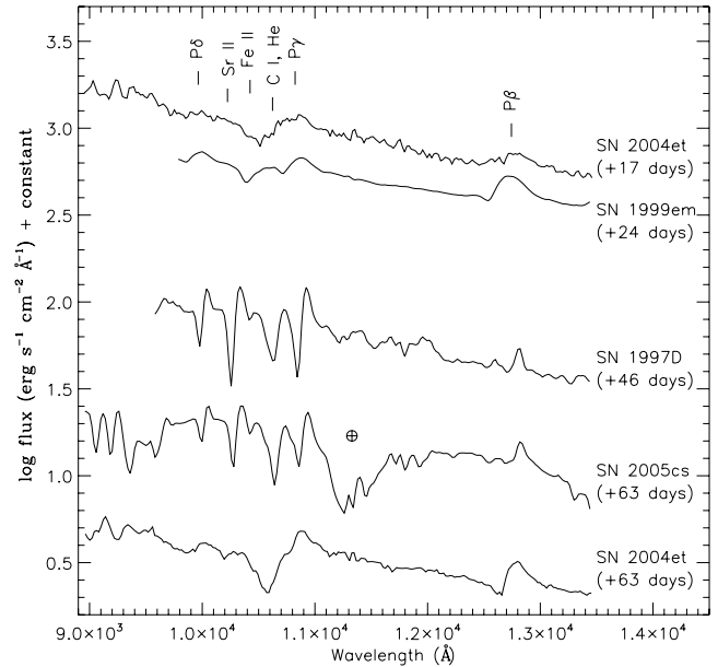
Figure 17. Comparison of the IJ -band spectra of SN 1999em, SN 1997D and SN 2005cs with two spectra of SN 2004et at epochs roughly matching the comparison SNe. The positions of the most prominent spectral features are marked.
