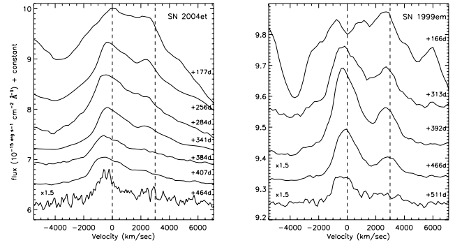
Figure 23. Evolution of the line profiles of [\text{O I}] 6300, 6364 Å for SN 2004et (left-hand panel) and for SN 1999em (right-hand panel). The vertical lines in the panels correspond to the zero velocities of the [\text{O I}] doublet at 6300, 6364 Å, respectively.
