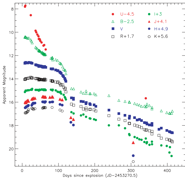
Figure 2. UBVRJHK light curves of SN 2004et, from soon after core collapse to +414 d post-explosion. The light curves are constructed using the data in Tables 1 and 2 and have not been corrected for reddening.
