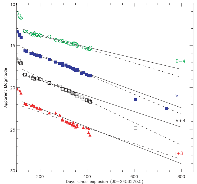
Figure 3. BVR light curves of SN 2004et during the tail phase. The solid lines indicate the decline rates calculated from \sim 136–300 d post-explosion, while the dashed lines indicate the decline rates calculated using the data from \sim 295–415 d. A steepening of the BVR light curves is seen while the slope of the I -band light curve becomes marginally less steep.
