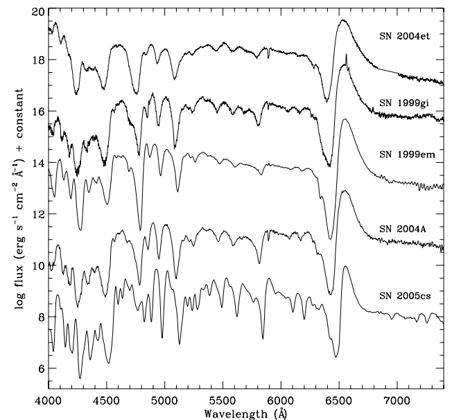
Figure 14. Comparison of coeval optical photospheric spectra of Type IIP SNe at \sim 39 d post-explosion. The spectrum of SN 2004et is taken from Sahu et al. (2006) and the spectrum of SN 2004A is from Appendix B. The other spectra are taken from the references given in Table 3.
