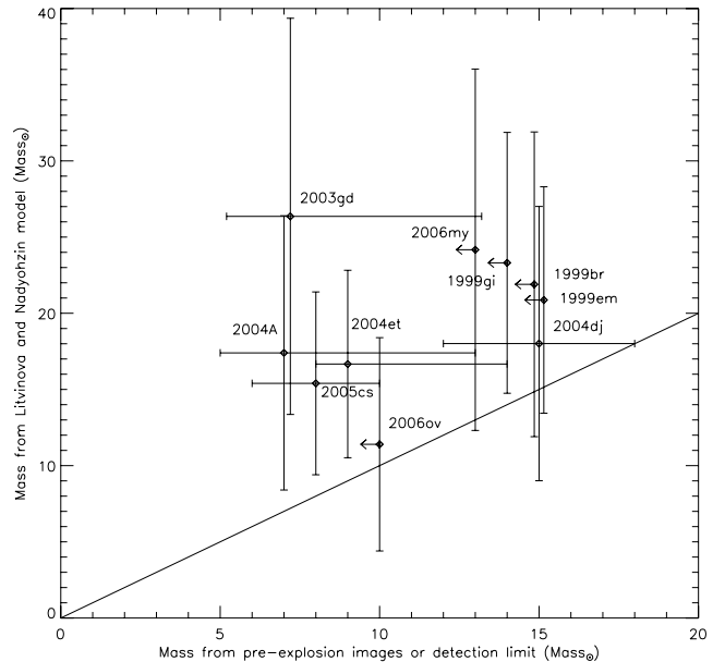
Figure 25. The progenitor masses obtained from the hydrodynamical equations of Litvinova & Naděžhin (1983, 1985) are plotted against the progenitor masses obtained from the pre-explosion images. Upper mass limits are plotted where detection limits have been set (Smartt et al. 2009). The values are given in Table 7, along with the associated errors. A one-to-one correspondence line is shown.
