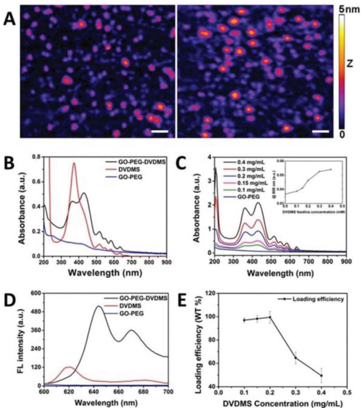
Fig. 1. (A) AFM image of GO-PEG and GO-PEG-DVDMS (white scale bar: 50 nm for X–Y dimension and the height is represented by the 5 nm Z-color bar). (B) UV-vis absorption spectra of GO-PEG (blue), DVDMS (red) and GO-PEG-DVDMS (black). (C) UV-vis absorption spectra of GO-PEG-DVDMS and the optical intensities changes at the wavelength 808 nm with different feeding concentrations of DVDMS ( C_{\text{GO-PEG}} = 0.1 \text{ mg mL}^{-1} ; C_{\text{DVDMS}} = 0.1\text{--}0.4 \text{ mg mL}^{-1} ). (D) The fluorescence spectra of GO-PEG (blue),
