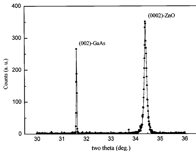
FIG. 1. The x-ray \theta - 2\theta rocking curve for a ZnO film on GaAs. A (0002)-ZnO peak indicates the c -axis oriented growth direction.
