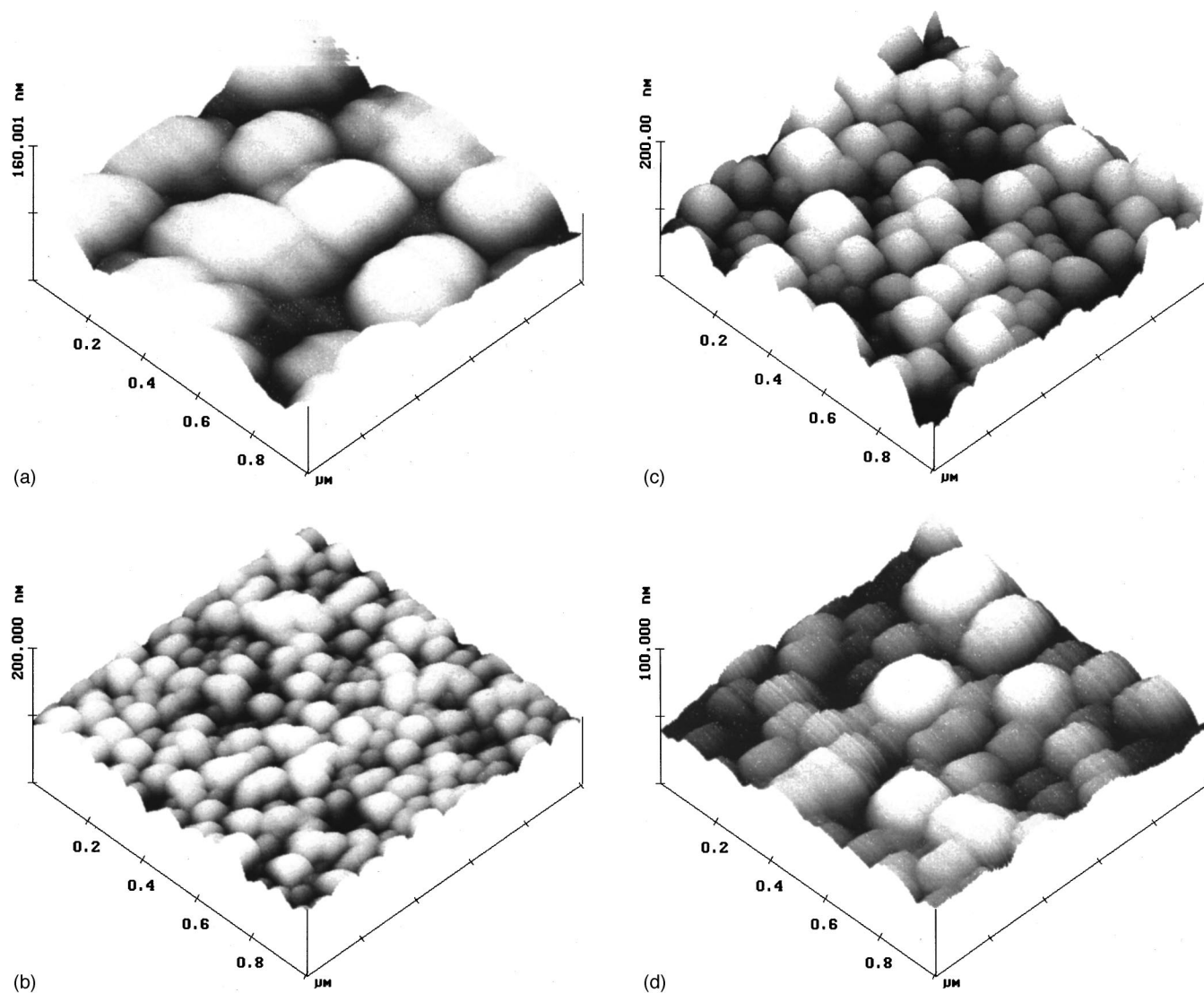
FIG. 3. AFM images of the ZnO films deposited by PLD. (a), (b), (c), and (d) are for ZnO samples grown at temperatures of 300, 350, 400, and 450 °C, respectively. The scanned area is 1 \times 1 \mu\text{m}^2 . The surface roughness for each is respectively 7.4, 9.4, 17.1, and 5.9 nm, proceeding from (a) to (d). The grain sizes of samples grown at 300 and 450 °C are larger than those of samples grown at 350 and 400 °C.
