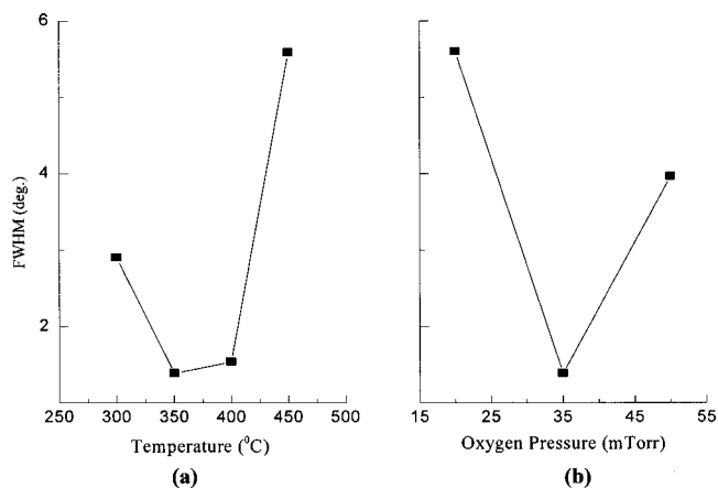
FIG. 2. (a) and (b) show the effects of growth temperature and oxygen gas pressure on the crystalline quality of ZnO film grown by PLD. The FWHM values of the x-ray \theta rocking curves are for the (0002)-ZnO peaks. The pressure of an ambient oxygen gas was fixed at 35 mTorr for (a) and the substrate temperature was fixed at 350 °C for (b). The best ZnO film was synthesized at 350 °C and 35 mTorr, with a FWHM value of 1.39° for the \theta rocking curve.
