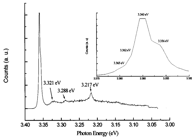
FIG. 4. PL spectra measured at 20 K obtained with a cw argon ion laser for a ZnO sample synthesized at a substrate temperature of 350 °C. The inset shows at least three different peaks in the photon energy range 3.35–3.37 eV.
