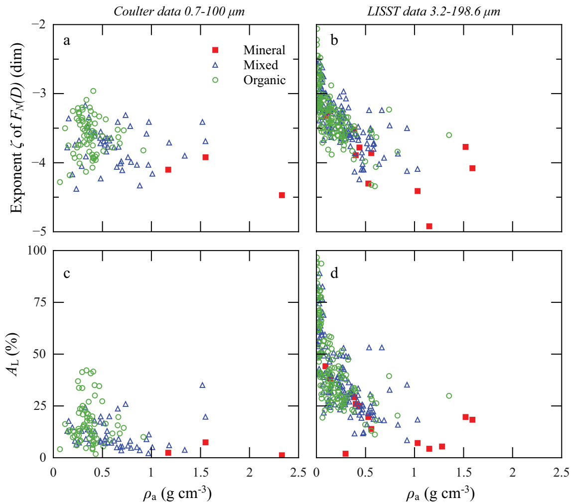
Fig. 7. Relationships between the power law slope of the PSD and apparent mean particle density for data calculated using the Coulter counter ( a ) or LISST ( b ) measurements. ( c, d ) Similar to panels a and b, but for the percentage of projected-area represented by particle diameters greater than 20 \mu\text{m} .
