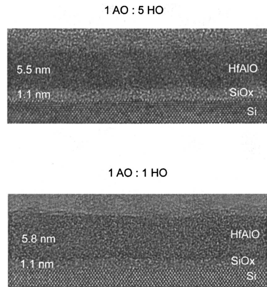
FIG. 1. HRTEM images for samples S5 and S9 used to determine the interface SiO 2 layer of thickness 11 Å in the SE data analysis.
