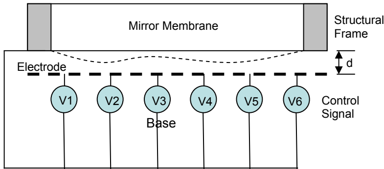
Figure 10. Mirror Membrane Deformable Mirror (MMDM)
