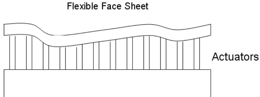
Figure 11. Simplified Piezo-electric Deformable Mirror Schematic
