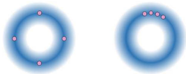
Figure 8: Diagrams showing nanoparticles trapped in the cross-section of a Laguerre-Gaussian beam. While, on symmetry grounds, it might be expected that the nanoparticles will settle at positions equidistant from each other (left-hand diagram), optical binding produces a clustering effect (right-hand diagram).
