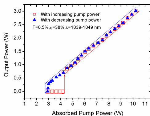
Fig. 1. Dependence of the output power of the Yb:LuVO 4 laser on the absorbed pump power, showing a sizable hysteresis loop.
