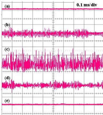
Fig. 2. Oscilloscope traces of the laser output showing the intensity fluctuations near the up-threshold. The traces from (a) to (e) were recorded when the pump power was decreased through the up-threshold point. The horizontal time scale is 0.1 ms/div.
