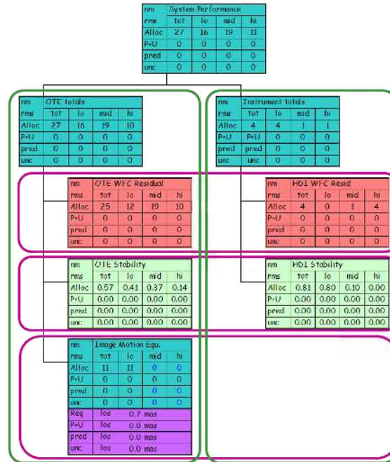
Figure 6. Highest level system budget arranged in a matrix fashion with components arranged by columns, and phenomena arranged by rows. Aspects of image motion cross component boundaries and is lumped under the telescope.
