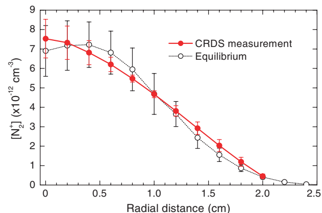
Figure 20. Concentration profiles of \text{N}_2^+ obtained by: (a) Abel-inversion of CRDS absorbance profile and (b) LTE calculation based on temperature profile obtained from Abel inverted absolute intensity profile of the 777.3 nm oxygen line.
