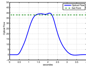
Fig. 5. Speed control results
