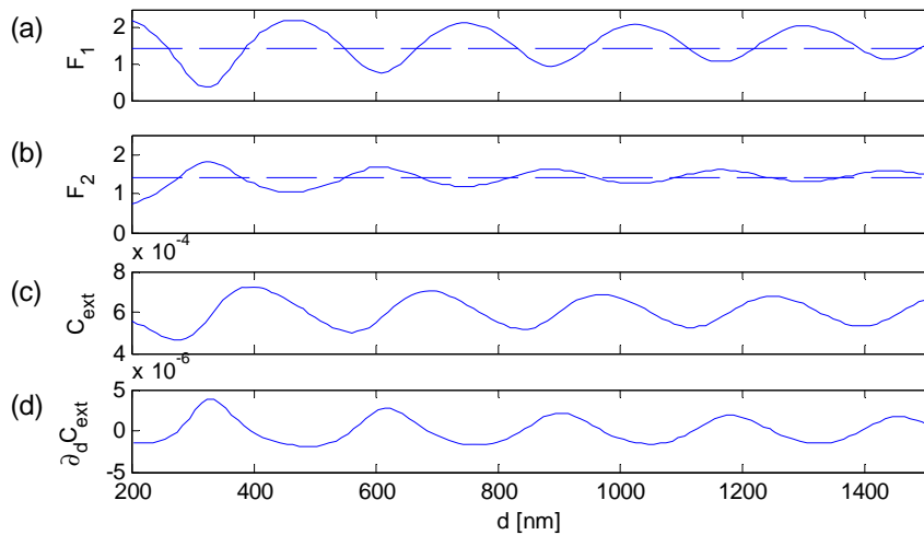
Fig. 8. (a) Forces on particle 1 and (b) particle 2; (c) extinction spectra and (d) derivative of the extinction, as a function of the distance d at the plasmon resonance wavelength \lambda = 550\text{ nm} .
