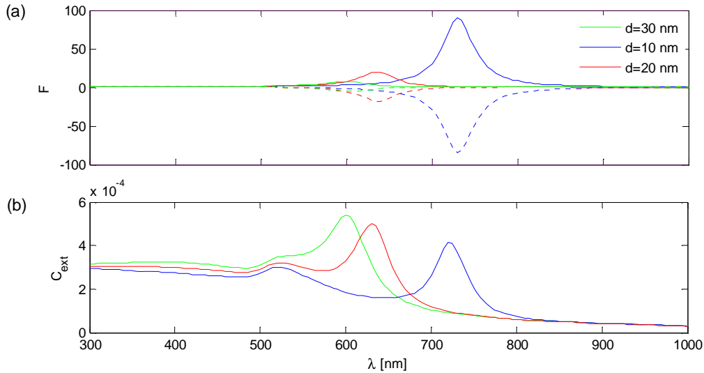
Fig. 4. (a) Forces on particle 1 (solid lines) and 2 (dashed lines) and (b) extinction spectra for three distances d in the near field coupling regime.
