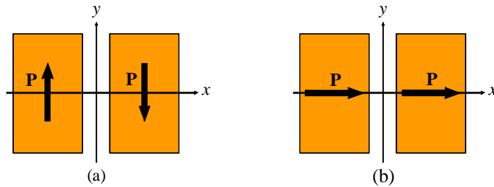
Fig. 5. Two coupling modes between both particles: (a) Antisymmetrical combination of both dipoles; this mode is non-radiative and produces a strong optical force. (b) Both particles are polarised along the incident field and no forces are observed.
