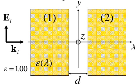
Fig. 1. Geometry of the system: two gold nanowires with the same rectangular section and a separation distance d are illuminated with a plane wave propagating in \mathbf{k}_i direction with incident field \mathbf{E}_i .
