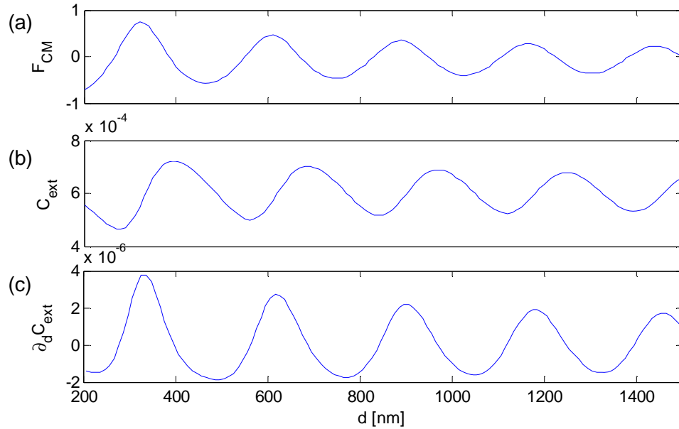
Fig. 11. (a) Force on particle (2) in the centre of mass reference frame at the plasmon resonance wavelength, (b) extinction and (c) extinction derivative, as a function of the separation distance d . Equilibrium positions F_{CM} = 0 are stable on the decreasing sides of the curve and unstable on the increasing sides.
