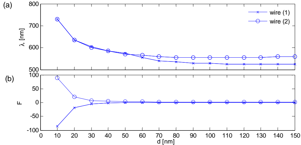
Fig. 6. (a) Resonance wavelength and (b) forces amplitude at the resonance for each particle, as a function of the separation distance d .
