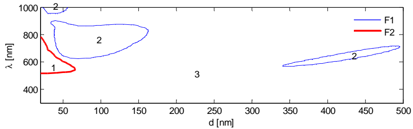
Fig. 3. The regions (1) (2) and (3) formed by blue and red contours determine the three possible interaction regimes between both nanowires as a function of the distance d and the wavelength \lambda : (1) Attractive forces, (2) Repulsive forces, (3) Positive forces.
