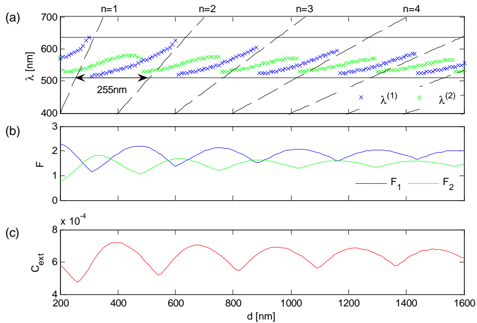
Fig. 9. (a) Evolution of force resonance wavelengths (b) force amplitudes and (c) extinction as a function of the separation distance d .
