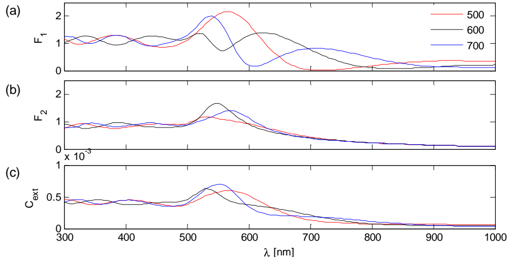
Fig. 7. (a) Forces on particle 1 and (b) particle 2, and extinction spectra for three distances d .
