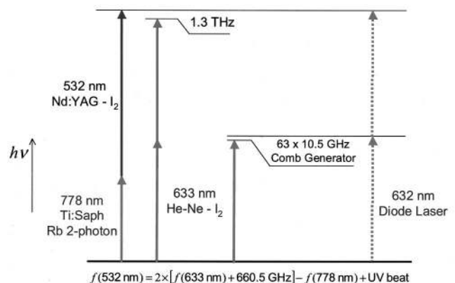
FIG. 3. Measurement of the iodine stabilized Nd:YAG laser frequency using the difference-frequency generation schemes, namely, frequency interval bisection and OFCG. The sum of the frequency of the doubled Nd:YAG laser and a Rb two photon stabilized Ti:S laser at 778 nm is about 1.3 THz higher than the doubled frequency of the iodine-stabilized 633 nm HeNe laser. This frequency gap can be bridged with an optical frequency comb generator based on a 632 nm diode laser (with the gap halved at 660 GHz).
