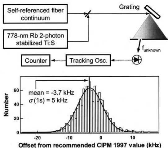
FIG. 21. Frequency measurement using the self-referenced comb. The diagram shows the experimental setup for measuring the two photon transition in ^{85}\text{Rb} using the self-referenced comb.
