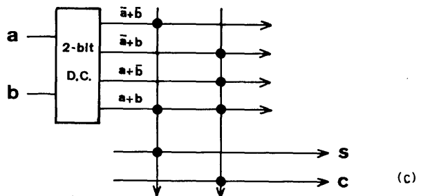
Fig. 2. Expressions of a half-adder circuit by (a) random logic, (b) array logic using 1-bit decoders, and (c) array logic using a 2-bit decoder.
