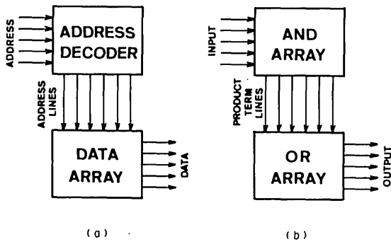
Fig. 1. Schematic diagrams of (a) electronic memory device and (b) logic array.
