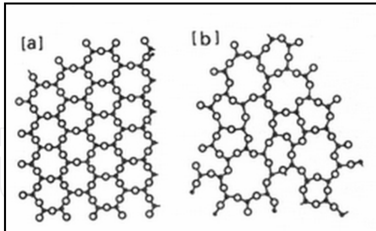
Fig. 6. Schematic 2-D representation of the structure of \text{SiO}_2 (a) crystalline (b) glassy form
