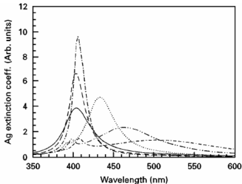
Fig. 5. Mie extinction coefficient of silver colloids of various radii as a function of wavelength of the incident light. R (nm): (—) 2.5, (---) 5, (- . -) 10, (.....) 25, (- - - -) 35, (- - . - -) 45.
