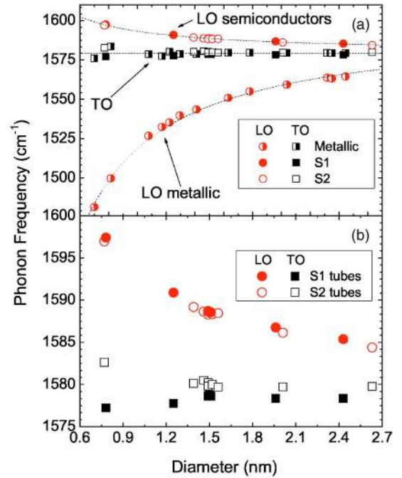
FIG. 8. (Color online) (a) Frequency of the LO and TO modes calculated by EZF-DFT at T_e=315 K. The LO phonons are in red; the TO phonons are in black. Different symbols identify metallic and semiconducting (S1 and S2) tubes. Dashed lines represent the fit of the EZF-DFT data, and correspond to the plot of Eq. (28). (b) LO and TO phonons of semiconducting tubes only. For S2 tubes TO phonon is \sim 2 \text{cm}^{-1} higher than in S1 tubes. No family dependence is observed for the LO phonon.
