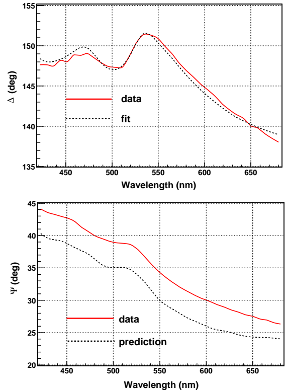
Fig. 8. Top: best fit (black dashed) to the measured average ellipsometric \Delta spectrum of the ETL 9102B (red solid), for the case of optical parameters fixed to n(440 \text{ nm}) = 2.7 , k(440 \text{ nm}) = 1.5 . Bottom: Measured average \Psi spectrum (red solid, not included in the global fit) and relevant prediction of the model giving the best global fit to V–W, VASRA and \Delta data (black dashed). The fits obtained after fixing (n, k) to the other considered values are very similar to the one shown here.
