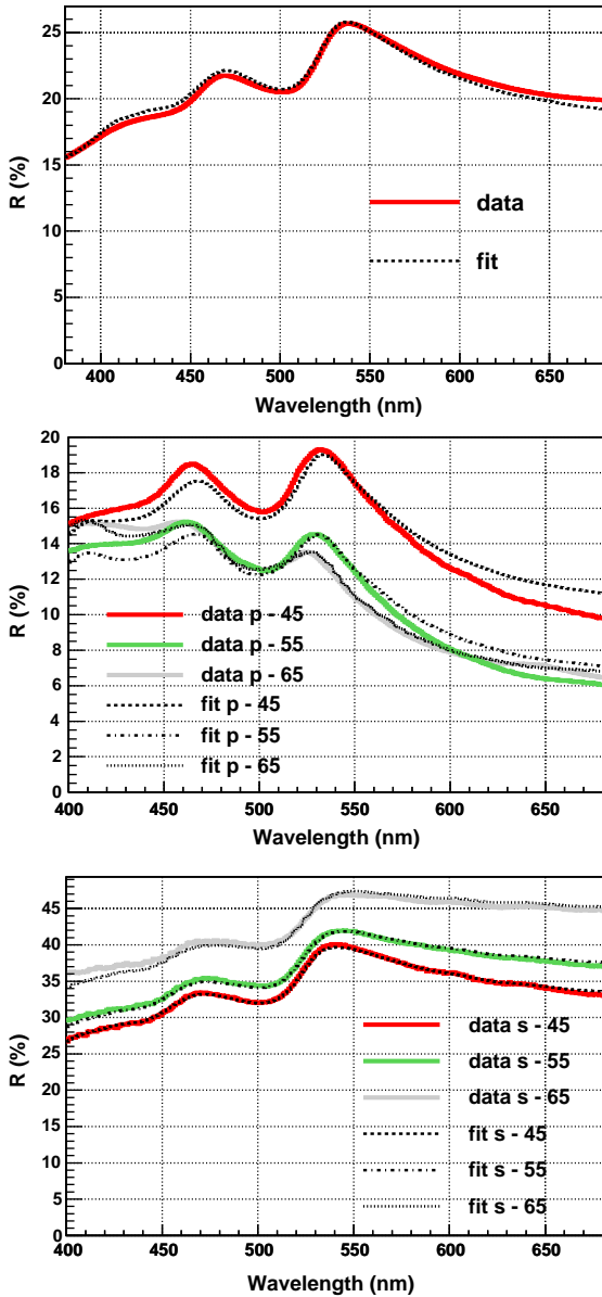
Fig. 7. Best global fit to the optical measurements of the ETL 9102B sample PMT, for the case of optical parameters fixed to n(440 \text{ nm}) = 2.7 , k(440 \text{ nm}) = 1.5 . Top: V–W absolute reflectance spectrum. Center: VASRA reflectance, parallel polarization. Bottom: VASRA reflectance, perpendicular polarization. The measurements are displayed in solid lines (see Figs. 4 and 5), the fits in dashed (dashed–dotted and dotted) lines. The fits obtained after fixing (n, k) to the other considered values are very similar to the one shown here.
