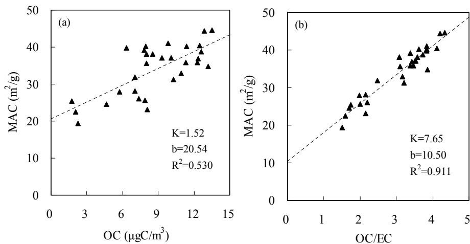
Fig. 3. Relationship between the MAC of EC and (a) the OC concentration, (b) the OC to EC ratio (OC/EC) during summer. Linear regression results are shown with K as the slope and b as the intercept. The trend was similar during winter.
