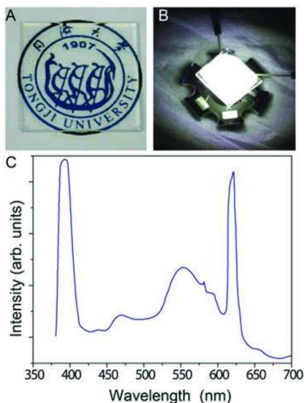
Figure 6. A) A photograph of MOF-PHEMA-3.5 hybrid materials. B) The hybrids bright white light emission under excitation by a 395 nm GaN chip and C) the corresponding LED electroluminescent spectrum. Reproduced with permission. [76] Copyright 2014, Royal Society of Chemistry.
