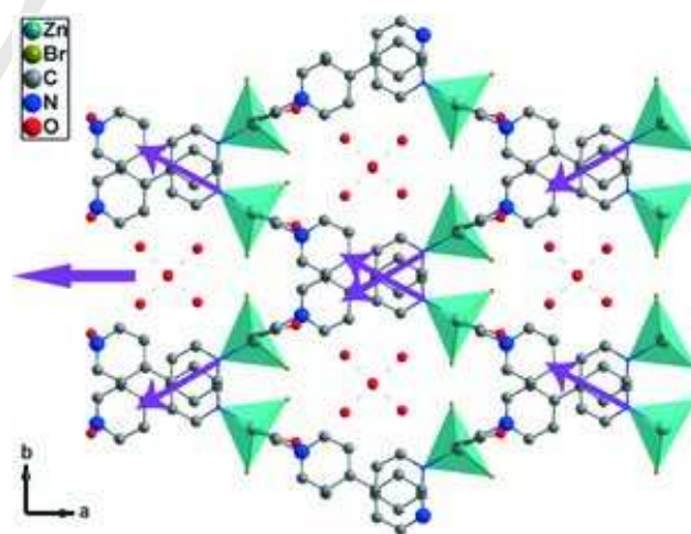
Figure 16. Molecular packing in a crystal of [ZnBr 2 (μ-CEbpy).3H 2 O] view along the c -axis. The violet arrows indicate the whole remnant polarity. Reproduced with permission. [184] Copyright 2014, Wiley-VCH.
