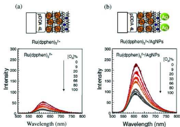
Figure 44. Hybrid polymer thin films with Ru(dpphen) 3 2+ and Ag NPs and the corresponding luminescence spectra showing the enhancement of the emission. Reproduced with permission. [523] Copyright 2015, Elsevier.
