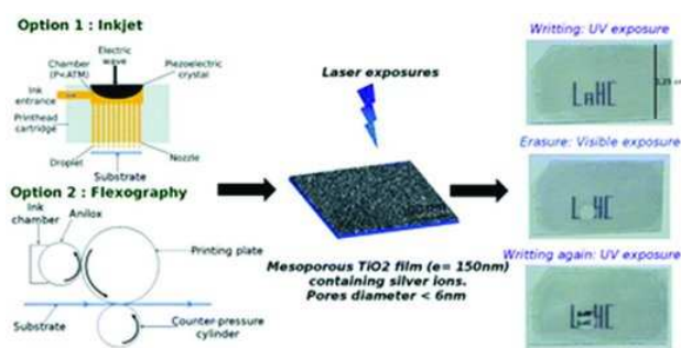
Figure 21. Principle of inkjet and flexography process (left), description of the Ag:TiO 2 material (center) and pictures of UV exposure inscription and visible exposure erasing on a film coated by flexography (right).
