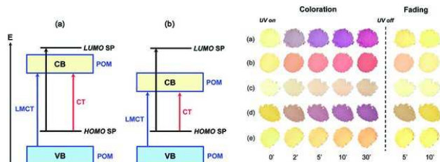
Figure 22. Schematic energetic diagrams displaying the three absorption phenomena predictable in SP-POM self-assembled structures when the SP cation is assembled with a POM unit having (a) a high-energy LMCT transition and (b) a low-energy LMCT transition. Photographs of powders of (a) \text{SP}_4\text{Mo}_8\cdot\text{CH}_3\text{CN} , (b) \text{SP}_4\text{Mo}_8\cdot\text{DMSO} , (c) \text{SP}_4\text{Mo}_8\cdot\text{DMF} , (d) \text{SP}_3\text{Mo}_8 , and (e) \text{SP}_2\text{AlMo}_6 at different time during the coloration process under UV irradiation (365 nm – 6 W), and the fading process under ambient light at room temperature. Reproduced with permission. [242] Copyright 2014, Royal Society of Chemistry.
