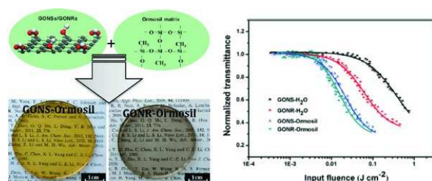
Figure 32. The GONS-Ormosil and GONR-Ormosil hybrid materials (left) and normalized transmittance versus the input fluence (right). Reproduced with permission. [376] Copyright 2014, Royal Society of Chemistry.
