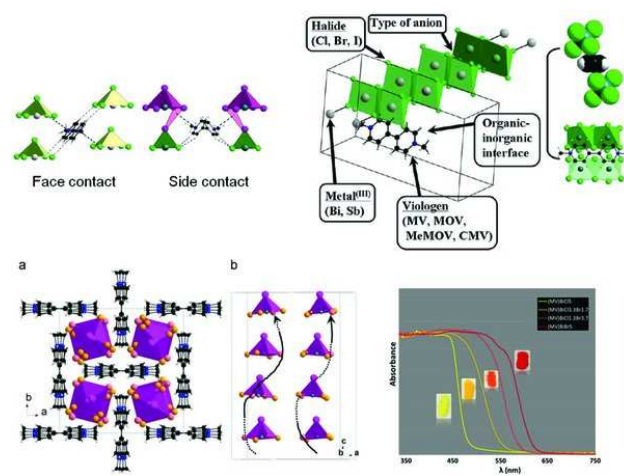
Figure 15. Top: (Left) Interactions at the organic-inorganic interface between one methylviologen cation and two anionic chains showing face and side contacts. (Right) Part of the structure of (MV)[Bi 2 Cl 8 ] showing one methylviologen entity and the inorganic network (left) and interactions between the organic cation and two inorganic anions (right: side view in space-filling representation and viewed along the direction perpendicular to the viologen plane), and the different parameters that can influence the photoinduced charge-transfer process in viologen halometalate salts. Reproduced with permission. [182] Copyright 2013, Wiley-VCH. Bottom: Structure of (MV)[SbBr 3.8 I 1.2 ] viewed along the chain axis showing the tetragonal arrangement (a), and syn coupling of two neighboring chains which displays opposite chiralities (b). UV-Vis spectra and pictures of (MV)[Bi 2 Cl 5-x Br x ] (x = 0, 3.7, 5) hybrids. Reproduced with permission. [183] Copyright 2012, Elsevier.
