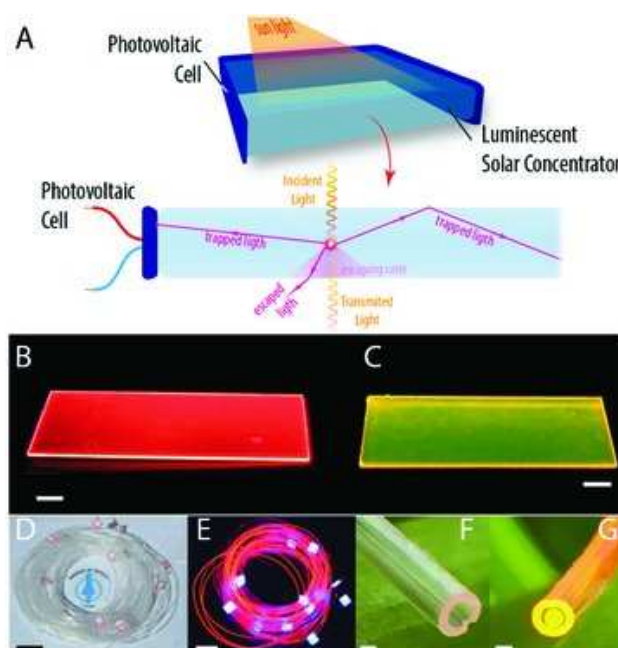
Figure 8. (A) Schematic representation of the working principle of a LSC. Photographs of two LSCs under UV irradiation (365 nm) based on (B) a di-ureasil hybrid doped with [Eu(btfa) 3 -(MeOH) 2 ] 2 bpta 2 , (bpta - = trans-1,2-bis(4-pyridil) ethane and MeOH = methanol) and (C) a tri-ureasil hybrid doped with PTMS (phenyltrimethoxysilane) and Rh6G. Photographs of meter-length Eu-based di-ureasil LSCs under (D) daylight conditions and (E) UV irradiation (scale bars of 10 -2 m). Detailed view of the Eu- (F) and Rh6G-based (G) LSCs extremities under outdoor illumination highlighting the light concentration (scale bars of 10 -3 m). Reproduced with permission. [101] Copyright 2016, RSC.
