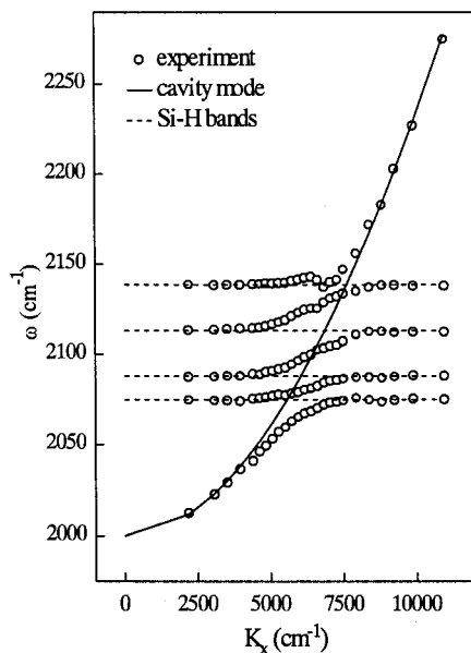
Fig. 1. Dispersion curves for the coupled mode between a PSi cavity and Si–H vibrations [13].
