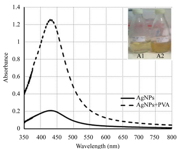
Figure 1. UV-Vis absorption spectra of colloidal silver nanoparticles synthesized and inserted photo synthesized silver nanoparticles.
