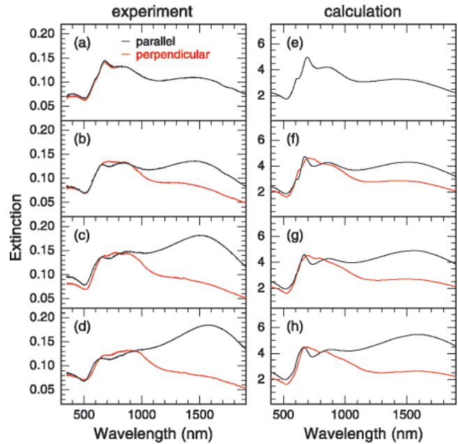
Figure 3. Measured and calculated optical extinction spectra for unpolarized light of spherical (a,e) and oblate spheroidal (b–d,f–h) Au-shell particles measured at an incidence angle of -45^\circ (black lines) and +45^\circ (red lines) to the sample normal, i.e., light incident approximately parallel or perpendicular to the spheroid minor axis. Size aspect ratios are 1.0 (a,e), 1.3 (b,f), 1.5 (c,g), and 1.7 (d,h).
