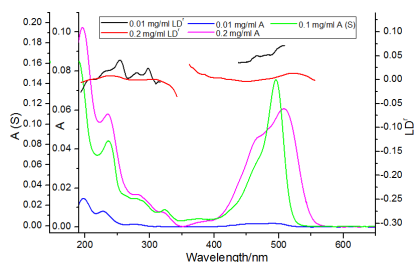
Figure 6 (a) LD spectra of fluorescein on PE OX deposited from solutions of concentrations indicated in the Figure. // and ⊥ indicate transition polarization with respect to the xanthere long axis in Figure 2. (b) Absorbance and LD' spectra of samples with concentrations 0.01 and 0.2 mg/ml overlaid with solution absorbance spectrum (S) and the dimer/monomer difference spectrum.
