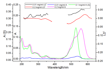
Figure 7 (a) LD spectra of rhodamine 6G on PE OX deposited from solutions of concentrations indicated in the Figure. // and ⊥ indicate transition polarization with respect to the xanthere long axis in Figure 2. (b) Absorbance and LD' spectra of samples with concentrations 0.01 and 0.2 mg/ml overlaid with solution absorbance spectrum (S) and the dimer/monomer difference spectrum.
