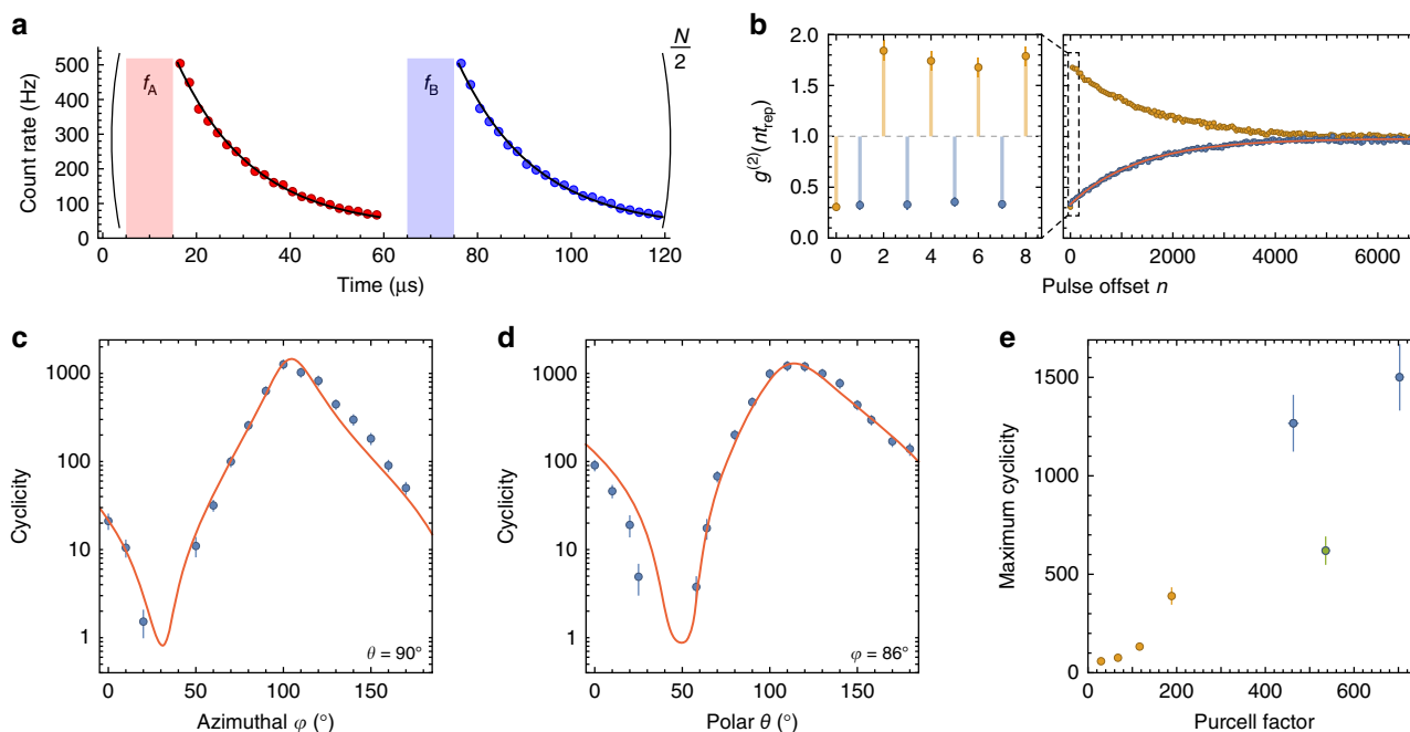
Fig. 2 Measuring the cyclicity of the optical transitions. a The measurement sequence consists of alternating pulses on the A and B transitions (10 \mu s) followed by a fluorescence collection window (45 \mu s), repeating every t_{rep} = 60 \mu s. The fluorescence lifetime is 16.2 \pm 0.2 \mu s, shortened from its free-space value of 11.4 ms by P = 703 \pm 6 in this device. b The intensity autocorrelation g^{(2)} is computed from the integrated fluorescence after each pulse. Odd values of n (blue points) probe the correlation between pulses driving different transitions and are anti-bunched as a result of the spin staying in the same state over many excitation cycles. g^{(2)} decays as e^{-n/n_0} because of optical pumping, giving the cyclicity C \approx n_0/2 . In this measurement, C = 660 \pm 66 . g^{(2)}(0) = 0.3 is consistent with the signal-to-background ratio of 10. c, d The cyclicity varies dramatically with the angle of the external magnetic field, but is described by a model (red line) based on the independently measured \mathbf{g} tensors (see text). e The cyclicity decreases rapidly with the Purcell factor, demonstrated here by measurements on several ions (shown in different colors) with the detuning varied to change P . In all plots, error bars denote estimated \pm 1\sigma statistical uncertainty.
