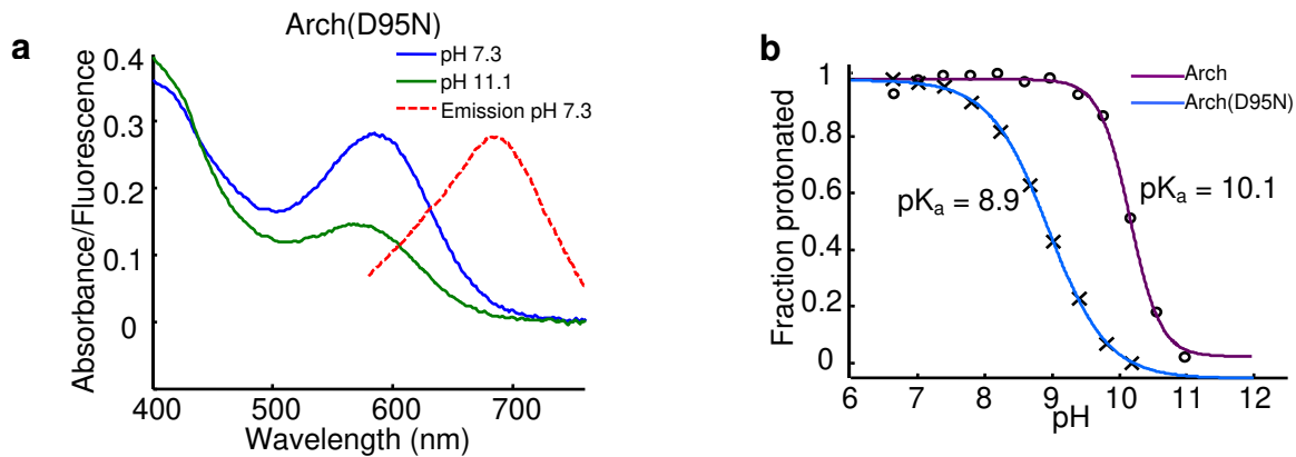
Supplementary Figure 1. pH-dependent spectra of Arch and Arch(D95N). (a) Arch(D95N) absorption at neutral (blue) and high (green) pH. At neutral pH, Arch(D95N) absorbed maximally at 585 nm. Fluorescence emission (red dashed line) was recorded on 2 \mu M protein solubilized in 1% DM, with \lambda_{exc} = 532 nm. (b) Absorption spectra were recorded on solubilized protein between pH 6 – 11. Singular Value Decomposition of absorption spectra between 400 – 750 nm was used to calculate the fraction of the SB in the protonated state as a function of pH. The result was fit to a Hill function to determine the pK_a of the SB.
