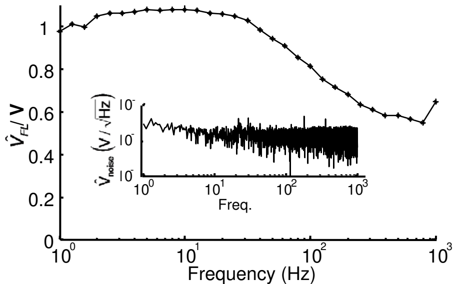
Supplementary Figure 3. Frequency response of Arch. A chirped sine wave with amplitude 50 mV and frequency from 1 Hz – 1 kHz was applied to the cell. Membrane potential \hat{V}_{FL} was determined from fluorescence and the Fourier transform of \hat{V}_{FL} was calculated. The uptick at 1 kHz is an artifact of electronic compensation circuitry. Inset: power spectrum of noise in \hat{V}_{FL} , under voltage clamp at constant V = 0 mV shows a shot-noise limited noise floor of 470 \mu\text{V}/(\text{Hz})^{1/2} at frequencies above 10 Hz. The noise figures reported here are specific to our imaging system and serve primarily as an indicator of the possible sensitivity of Arch.
