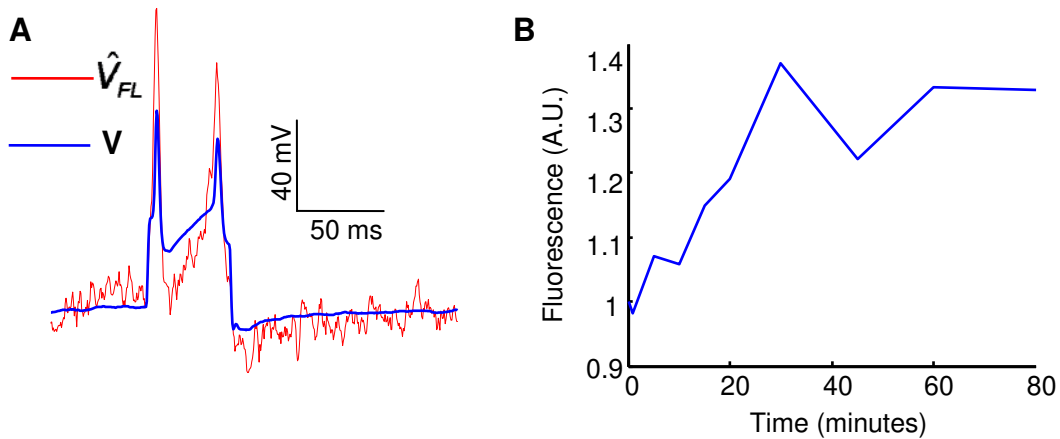
Supplementary Figure 6. Arch reports action potentials without exogenous retinal. A) Single-trial recording of APs from a 14 DIV neuron expressing Arch, without exogenous retinal, showing electrical (blue) and fluorescence (red) traces. APs are clearly resolved. B) Fluorescence of a single neuron as a function of time after addition of 10 \mu M retinal. To avoid conflation of voltage dynamics with the effects of retinal incorporation, the neuron was depolarized by treatment with CCCP prior to the experiment.
