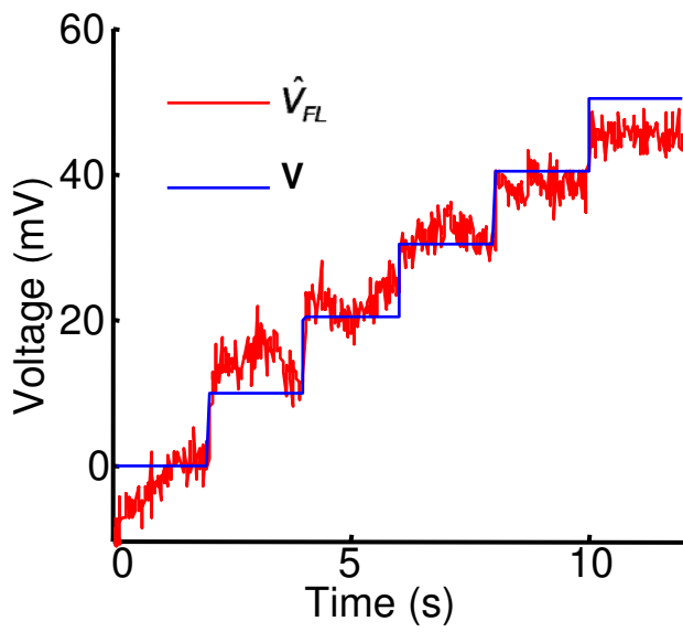
Supplementary Figure 4. Sensitivity of Arch to voltage steps of 10 mV. Whole-cell membrane potential determined via direct voltage recording, V , (blue) and weighted Arch fluorescence, \hat{V}_{FL} , (red).
