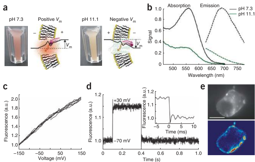
Figure 1 | Arch is a fluorescent voltage indicator. (a) Model of Arch as a voltage sensor, in which pH and membrane potential can both alter the protonation of the Schiff base. The cuvettes contain intact E. coli expressing Arch. (b) Absorption and fluorescence emission spectra of Arch at neutral and high pH. (c) Fluorescence of Arch (divided by the value at -150 mV) as a function of membrane potential (recorded over six consecutive sweeps). (d) Dynamic response of Arch to steps in membrane potential between -70 mV and +30 mV. The overshoots on the rising and falling edges were an artifact of electronic compensation circuitry. The smaller amplitude compared to c is because background subtraction was not performed in d. Data were averaged over 20 cycles. Inset, step response occurred in less than the 500 \mu s resolution of the imaging system. (e) Fluorescence micrograph of an HEK 293 cell expressing Arch (top) and pixel-weight matrix showing regions of voltage-dependent fluorescence (bottom). a.u., arbitrary units. Scale bar, 10 \mu m.
