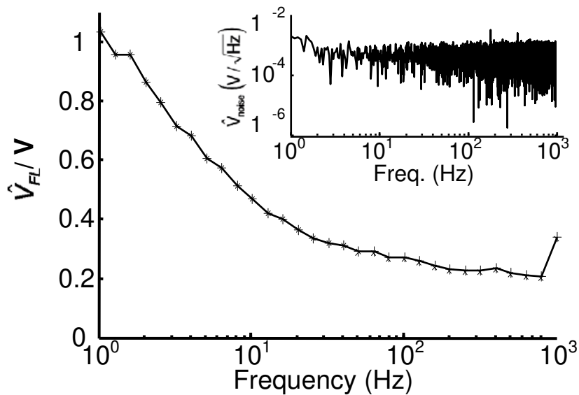
Supplementary Figure 7. Frequency response of Arch(D95N), measured in the same manner as for Arch (Supplementary Fig. 2).
