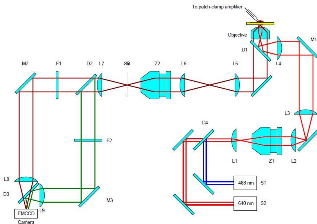
Supplementary Figure 2. Diagram of fluorescence microscope
