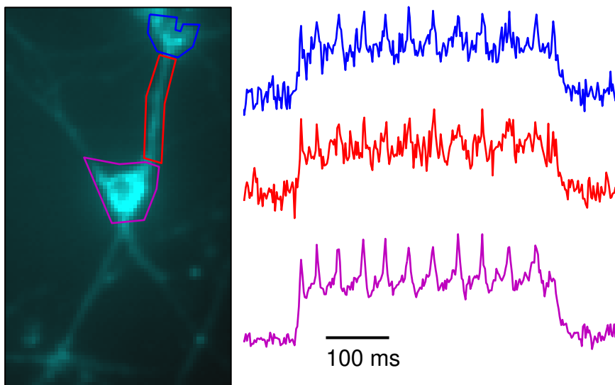
Supplementary Figure 5. Sub-cellular localization of action potentials on a single-trial basis. The vertical scale on the fluorescence traces is arbitrary. The lower regions of the cell, shown in Fig. 2e, did not have adequate SNR to indicate APs on a single-trial basis.
