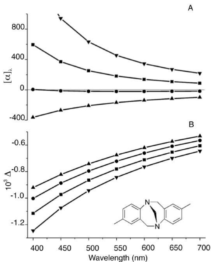
Figure 8. ORD (A) and depolarized right-angle ICP RayOA curves (B) of (+)-(5 S , 11 S )- Tröger's base calculated using HF ( \blacktriangle ) and DFT with B3LYP ( \blacksquare ), B3LYP ( \bullet ), BLYP ( \blacktriangledown ) functionals. Calculations used the 6-31G* basis set with the B3LYP/6-311G** optimized geometry. The predicted ORD curves show significant variation depending on the choice of the QM method. In contrast, the RayOA curves are uniformly negative in sign and possess nearly identical curvatures. 68
