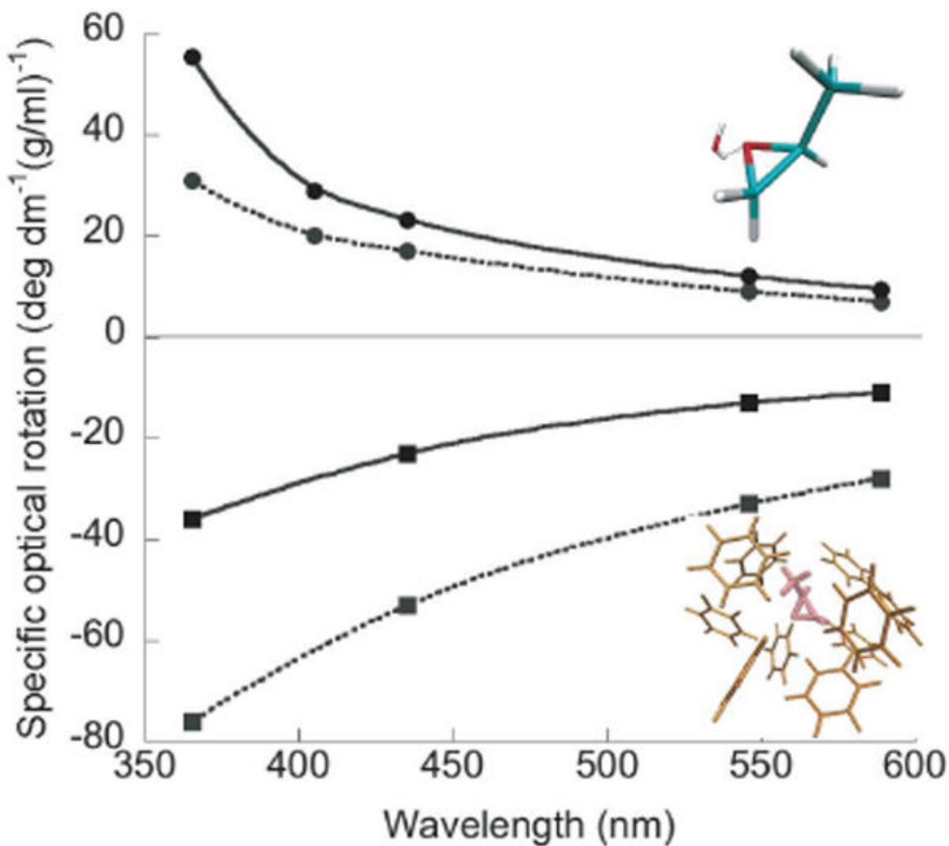
Figure 5. Measured (dashed line) and computed (solid line) ORD of ( S )-methyloxirane in water (●) and benzene (■). The hydrogen bonded methyloxirane-water adduct (top structure) dominates the ORD in aqueous solution. 40 In contrast, the chiral benzene cluster (bottom structure) dominates the ORD in benzene. 39,45
