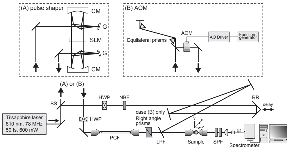
Fig. 8. Experimental setup for broadband CARS spectroscopy using a pulse shaper (A) and an AOM (B). Here, BS: beam splitter, RR: retroreflector, CM: concave mirror, G: grating, HWP: half-wave plate, NBF: narrow bandpass filter, SPF: short-wavelength pass filter, and LPF: long-wavelength pass filter.
