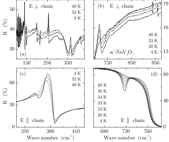
FIG. 9. Detailed temperature dependence of some of the zone boundary folded modes observed in the reflectivity spectra, for T < T_c , with E \perp chain (a,b) and E \parallel chain (c,d).
