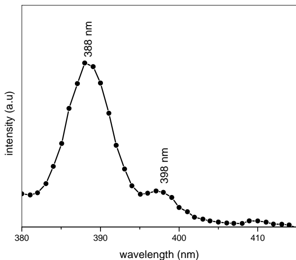
Fig. 5 The room temperature PL emission spectra of ZnS nanoparticles
