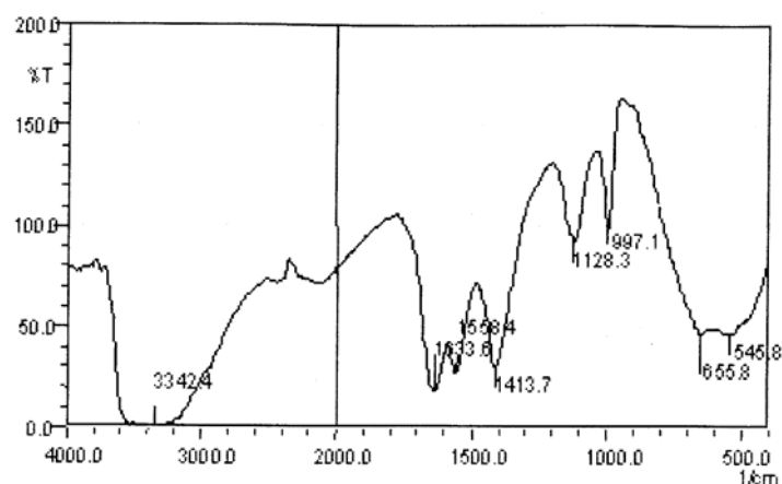
Fig. 3 FTIR spectrum of ZnS nanoparticles
