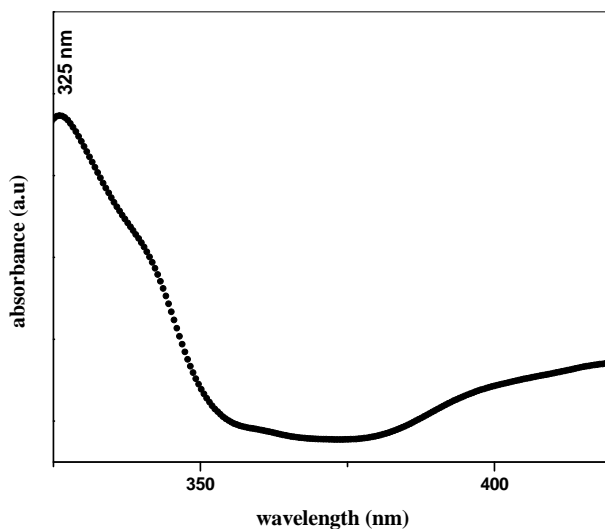
Fig. 4 UV Spectra of ZnS nanoparticles.
