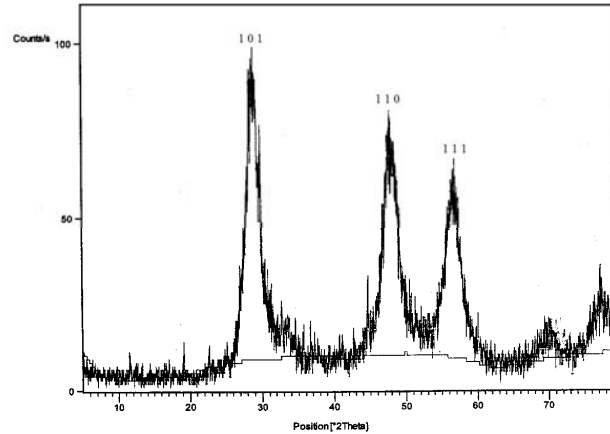
Fig. 1 XRD pattern of ZnS nanoparticles.
