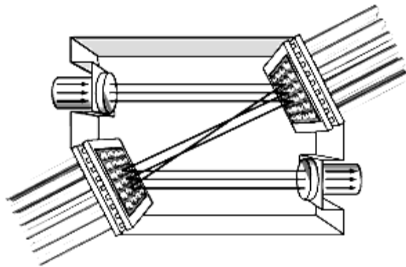
Figure 3.2 – Two arrays of N tilting mirrors, interconnecting N inputs with N outputs
