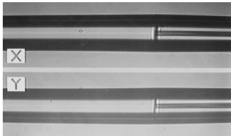
Figure 6.28 – Visualization of the SMF-28 TM /PCF splice in the Fujikura’s FSM-40S screen.
