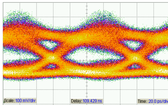
Figure 7.7 – Eye Diagram of the output of the OADM when \lambda_2 is added to the system when \lambda_1 and \lambda_3 are at the input port
