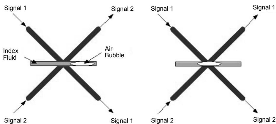
Figure 3.7 – Principle of operation of a 2 × 2 bubble switch. (left) bar state; (right) cross state.
