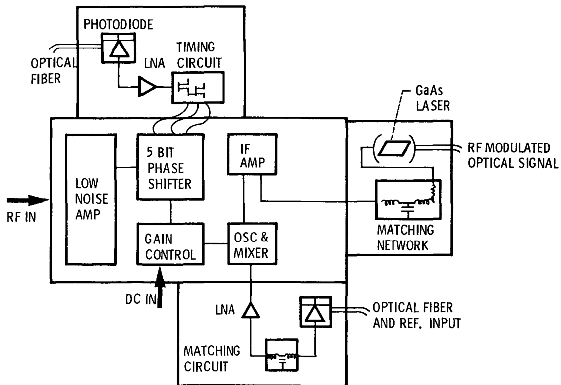
Figure 7. - Optical integrated circuits interfaced with MMIC receive module for optical fiber interconnections.
