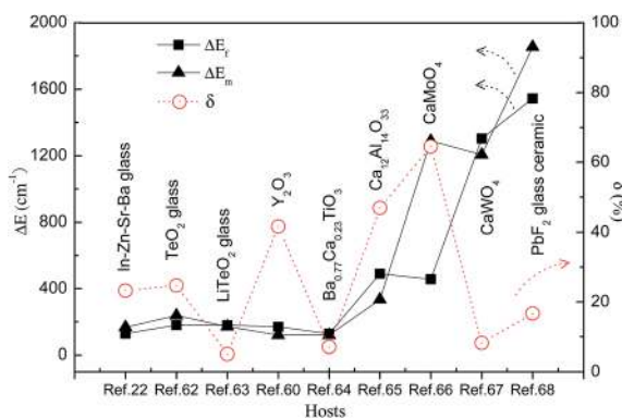
Fig. 11 Host dependent \Delta E_x and \Delta E_m between the TCL of Ho 3+ ions, and the corresponding \delta values.
