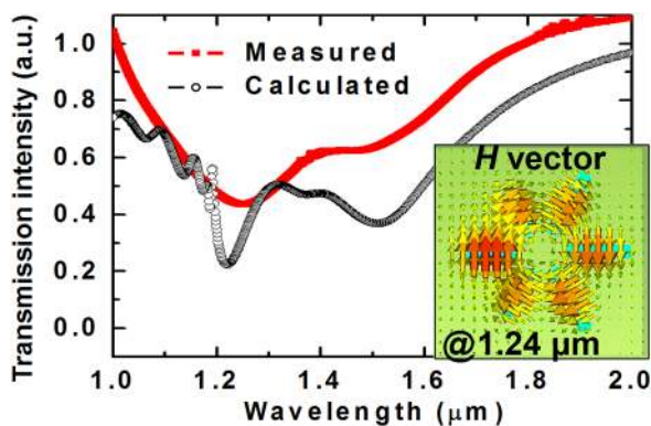
FIG. 2. Transmission spectra of the toroidal structure from both experiment and simulation. The inset shows the H -vortex distribution at the toroidal resonant mode (enhanced online) [URL: http://dx.doi.org/10.1063/1.4757613.1 ].
