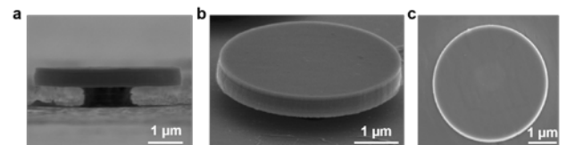
Figure 2. SEM images of a 4- \mu\text{m} fabricated micro-disk. (a) 90° tilted view of the disk, showing vertical profile. (b) 70° tilted view of the disk, revealing smooth sidewall. (c) top-down view of the disk, showing its circular geometry.
