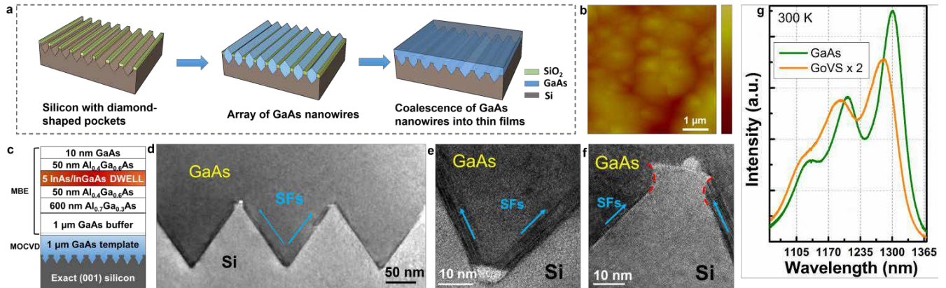
Figure 1 Epitaxial InAs QDs micro-disks on GoVS substrate. (a) Procedure of growing antiphase-domain-free GaAs thin films out of highly ordered, array of planar GaAs nanowires on silicon substrates with diamond-shaped pockets. (b) AFM image of approximately 1 \mu\text{m} coalesced GaAs thin film grown on the nanowire arrays. The vertical bar is 25 nm. (c) Schematic of the as-grown structure of micro-disk lasers. (d)-(f) Cross-sectional TEM image of the V-grooved structure, showing stacking faults (indicated by the blue arrows) trapped by the Si pockets. (g) Room temperature photoluminescence spectra of the as-grown structures on the GoVS template and a GaAs substrate at a pump power density of 4.7 \text{kW}/\text{cm}^2 .
