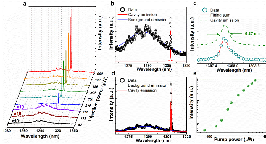
Figure 3. Laser operation of a 4- \mu\text{m} diameter micro-disk on GoVS. (a) PL spectra taken at increasing pump powers. (b) Sub-threshold spectrum (165 \mu\text{W} ). The symbols represent measured data, the blue line is a fit to the broad InAs QDs photoluminescence spectrum background, the red line is a fit to the narrow cavity emission. (c) High-resolution spectrum at 165 \mu\text{W} . The symbols represent measured data, the red line is a fitting sum of the measured data using bi-Lorentzian curves, and the green line is a fit to the narrow cavity emission. (d) Above-threshold spectrum (248 \mu\text{W} ). The symbols represent measured data, the blue line is a fit to the broad InAs QDs photoluminescence spectrum background, the red line is a fit to the narrow cavity emission. (e) Integrated photoluminescence intensity of the dominant mode as a function of pump power in the log-log scale.
