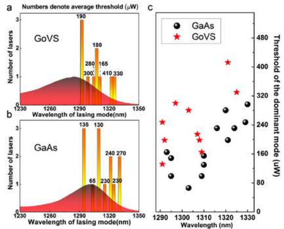
Figure 4. Statistical analysis of lasing behavior of micro-disks fabricated on GoVS and GaAs. (a), (b) Histogram of the lasing wavelength for each measured device on GoVS and GaAs, respectively. The average lasing threshold of the devices within each histogram bar is denoted by the number displayed on top of it. The normalized photoluminescence spectrum of the un-processed sample is denoted in red. (c) Lasing threshold is plotted as a function of a lasing wavelength for micro-disks fabricated on GoVS (red stars) and GaAs (black spheres).
