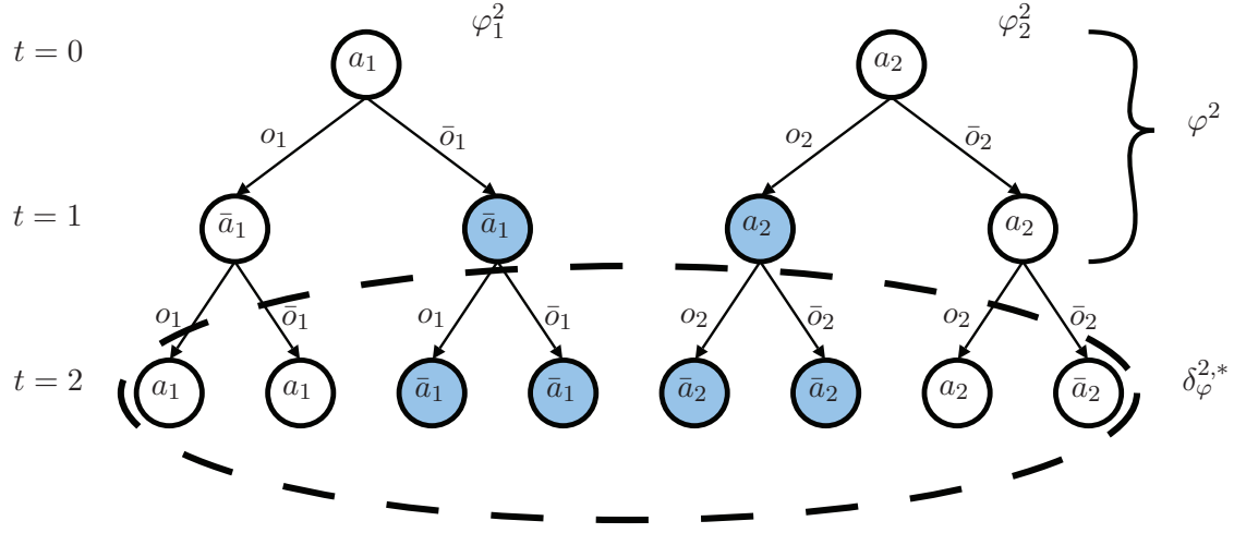
Figure 7: Computation of sequential rational Q^* . \delta_{\varphi}^{2,*} is the optimal decision rule for stage t = 2 , given that \varphi^2 is followed for the first two stages. Q^*(\vec{\theta}^1, \varphi^2) entries are computed by propagating relevant Q^* -values of the next stage. For instance, for the highlighted joint history \vec{\theta}^1 = \langle (a_1, \bar{o}_1), (a_2, o_2) \rangle , the Q^* -value under \varphi^2 is computed by propagating the values of the four successor joint histories, as per (4.20).
