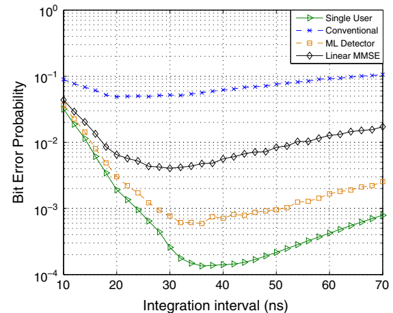
Figure 3. Bit error probability versus |\Gamma| for CM4 with N_f = 4 and N_c = 250 at a signal-to-noise ratio of 12 dB.
