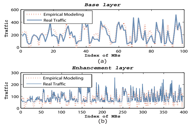
Fig. 5. Comparison of traffic between the empirical model and the real encoded traffic for base layer (a) and enhancement layer (b) of the 1 st sequence of ‘Akiyo’
