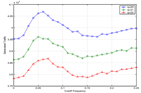
Fig. 8. The total traffic of the layered coding scheme as a function of cutoff frequency
