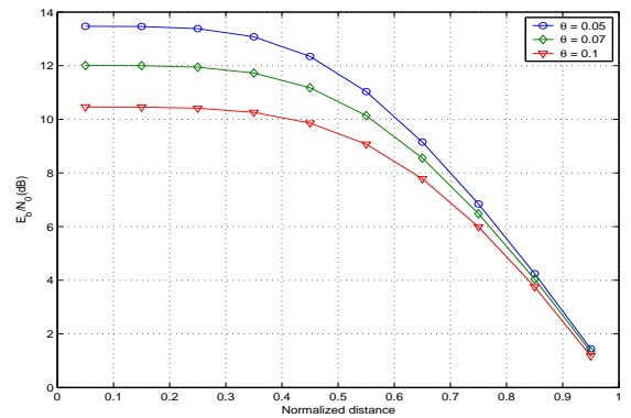
Fig. 9. E_b/N_0 as a function of normalized distance for orthogonal parameters
