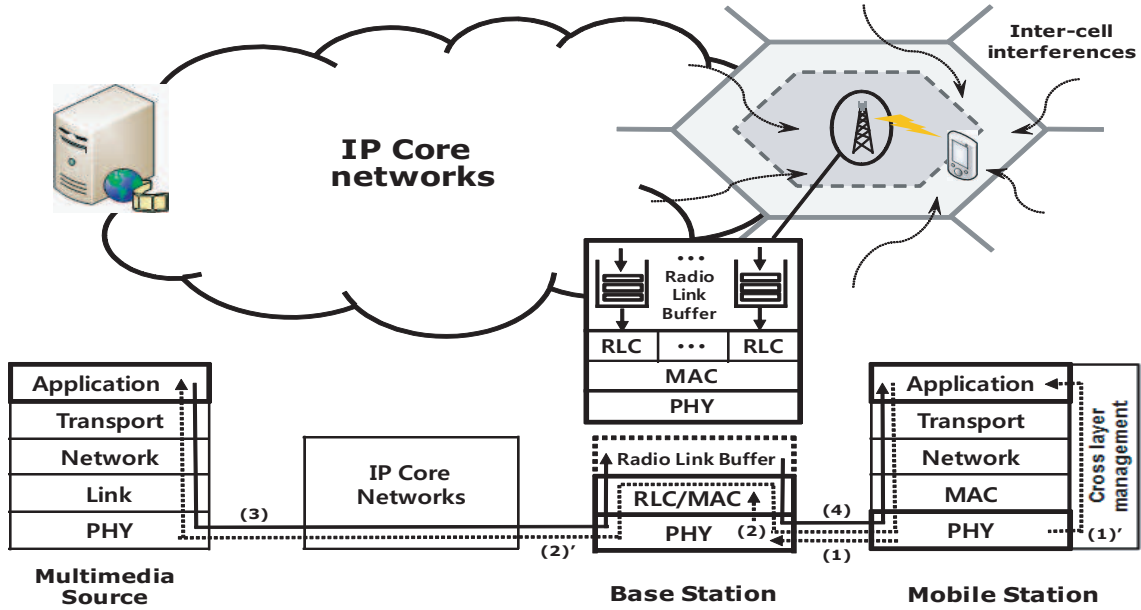
Fig. 1. Signal flows through network nodes and protocol stacks for the cross-layer design
