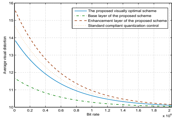
Fig. 7. Average visual distortion as a function of target bit rate
