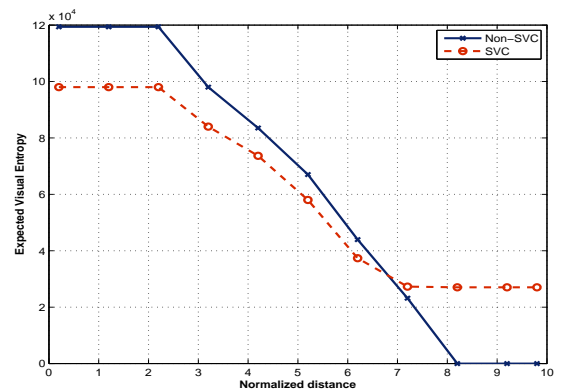
Fig. 10. The expected visual entropy as a function of normalized distance for the intra-frame
